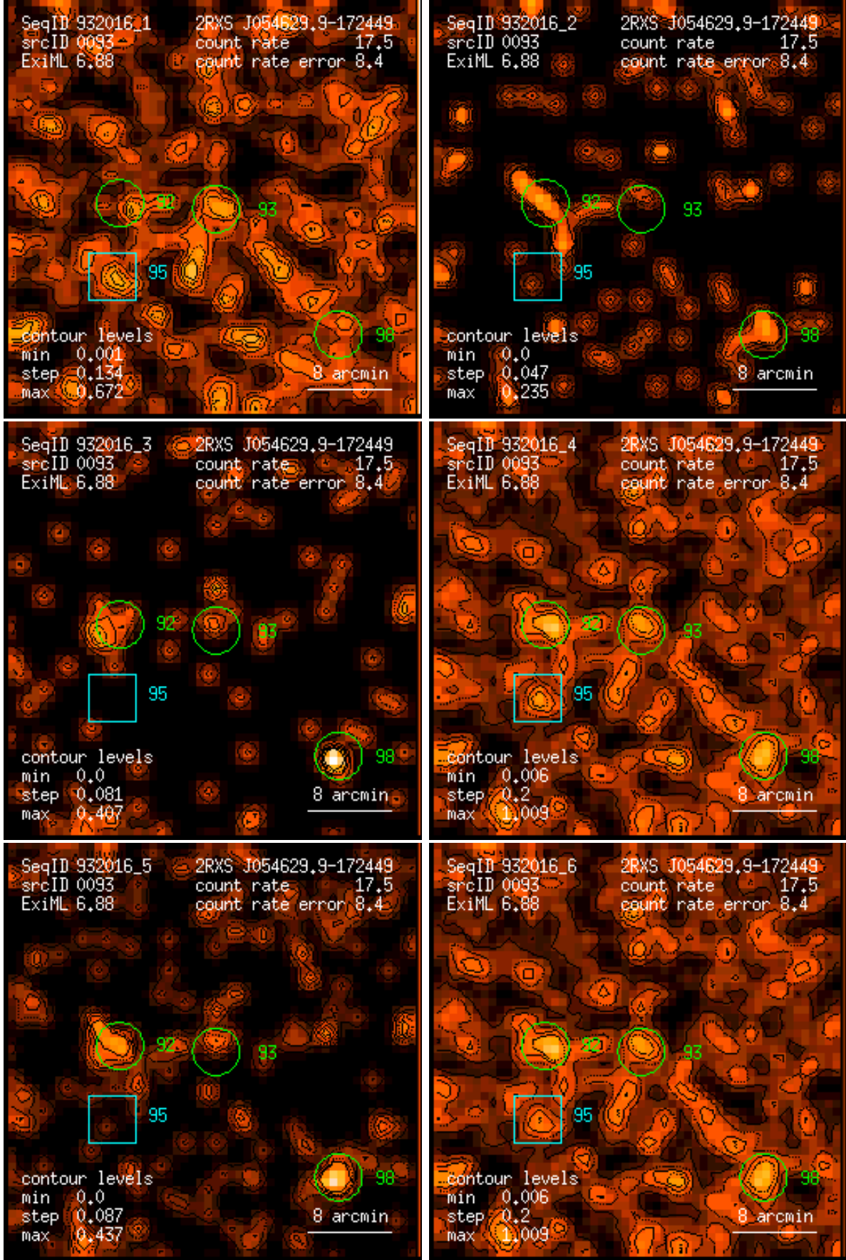
Figure 93: RASS 932016: detection 0093: band rate images, Gaussian filter: (1) PSPC channels 11 – 41, (2) 52 – 90, (3) 91 – 201, (4) 11 – 235, (5) 52 – 201, (6) 11 – 201. Broad band rates in counts/ks. Band rate contour levels in counts/ks/arcmin 2 .
