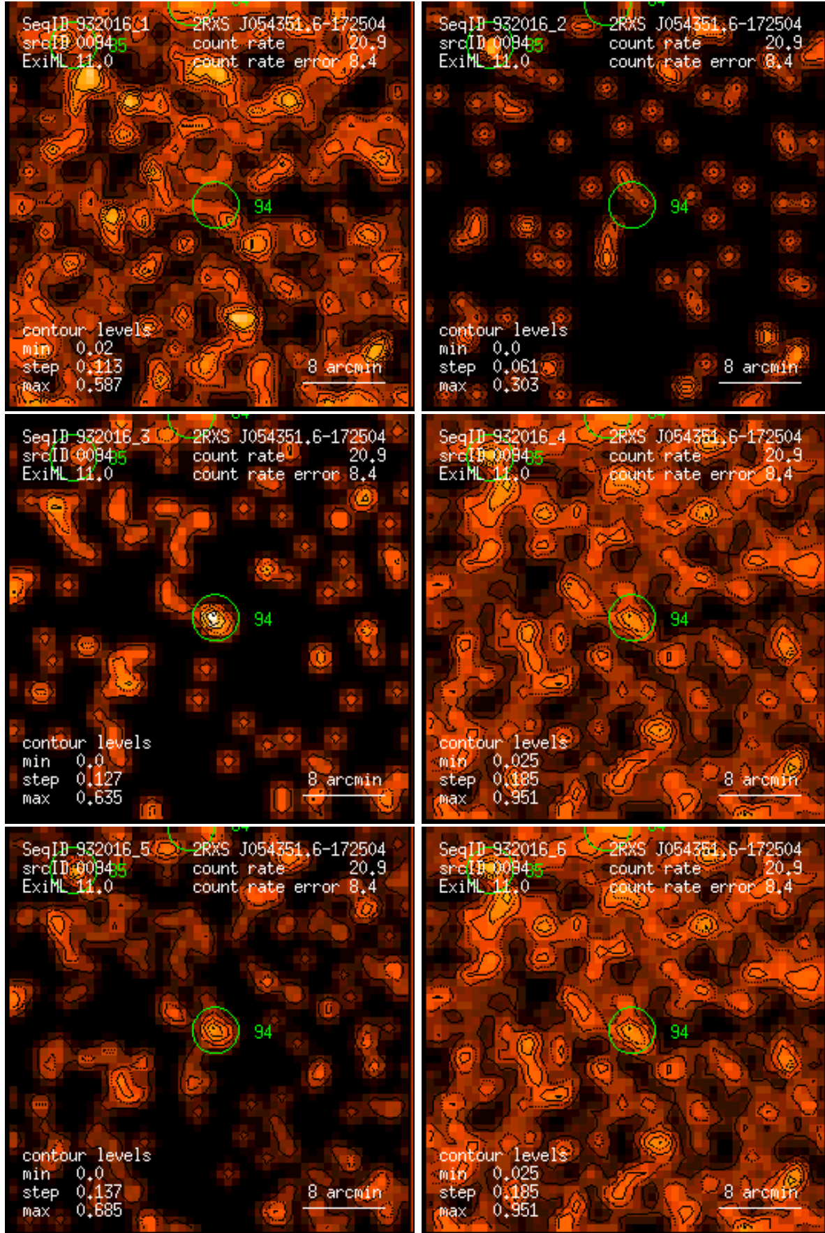
Figure 94: RASS 932016: detection 0094: band rate images, Gaussian filter: (1) PSPC channels 11 – 41, (2) 52 – 90, (3) 91 – 201, (4) 11 – 235, (5) 52 – 201, (6) 11 – 201. Broad band rates in counts/ks. Band rate contour levels in counts/ks/arcmin 2 .
