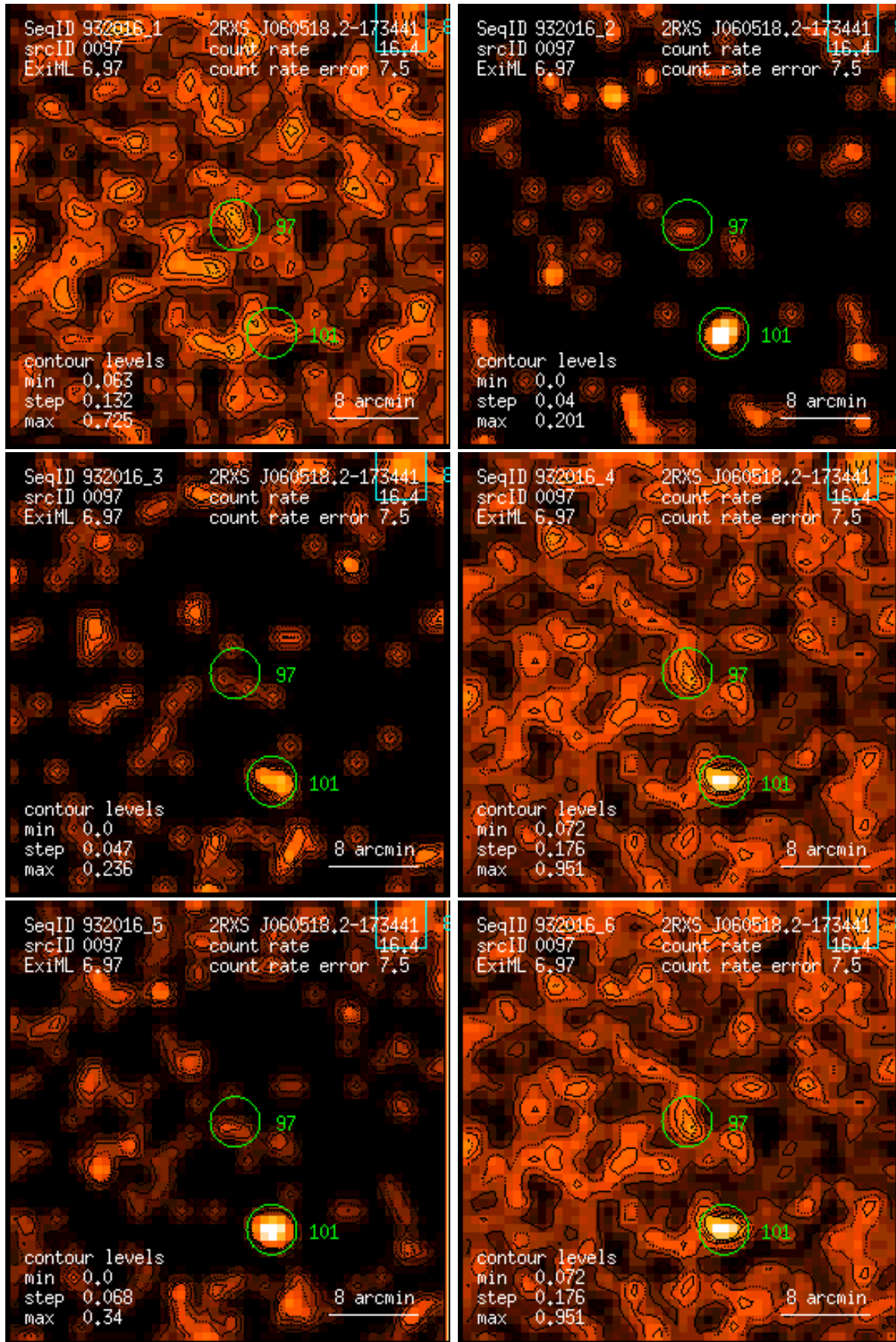
Figure 97: RASS 932016: detection 0097: band rate images, Gaussian filter: (1) PSPC channels 11 – 41, (2) 52 – 90, (3) 91 – 201, (4) 11 – 235, (5) 52 – 201, (6) 11 – 201. Broad band rates in counts/ks. Band rate contour levels in counts/ks/arcmin 2 .
