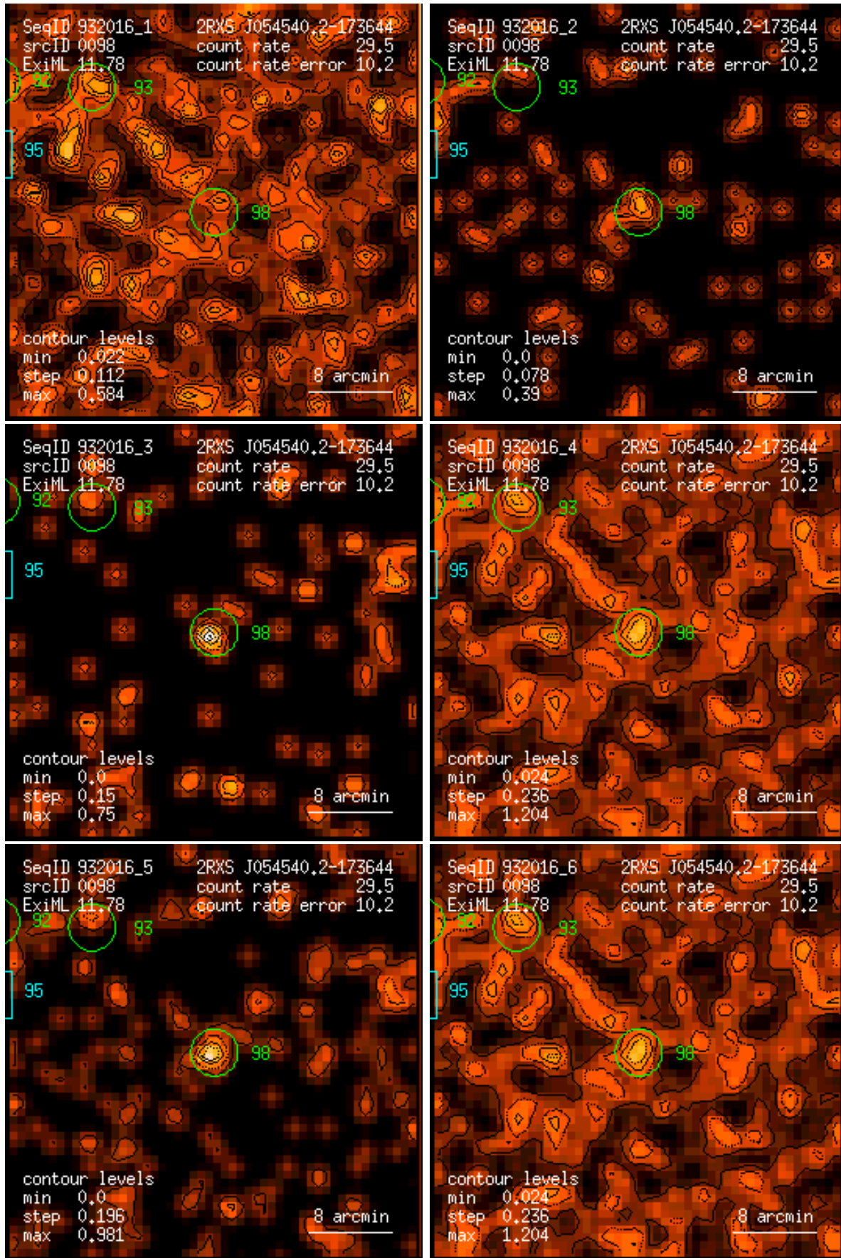
Figure 98: RASS 932016: detection 0098: band rate images, Gaussian filter: (1) PSPC channels 11 – 41, (2) 52 – 90, (3) 91 – 201, (4) 11 – 235, (5) 52 – 201, (6) 11 – 201. Broad band rates in counts/ks. Band rate contour levels in counts/ks/arcmin 2 .
