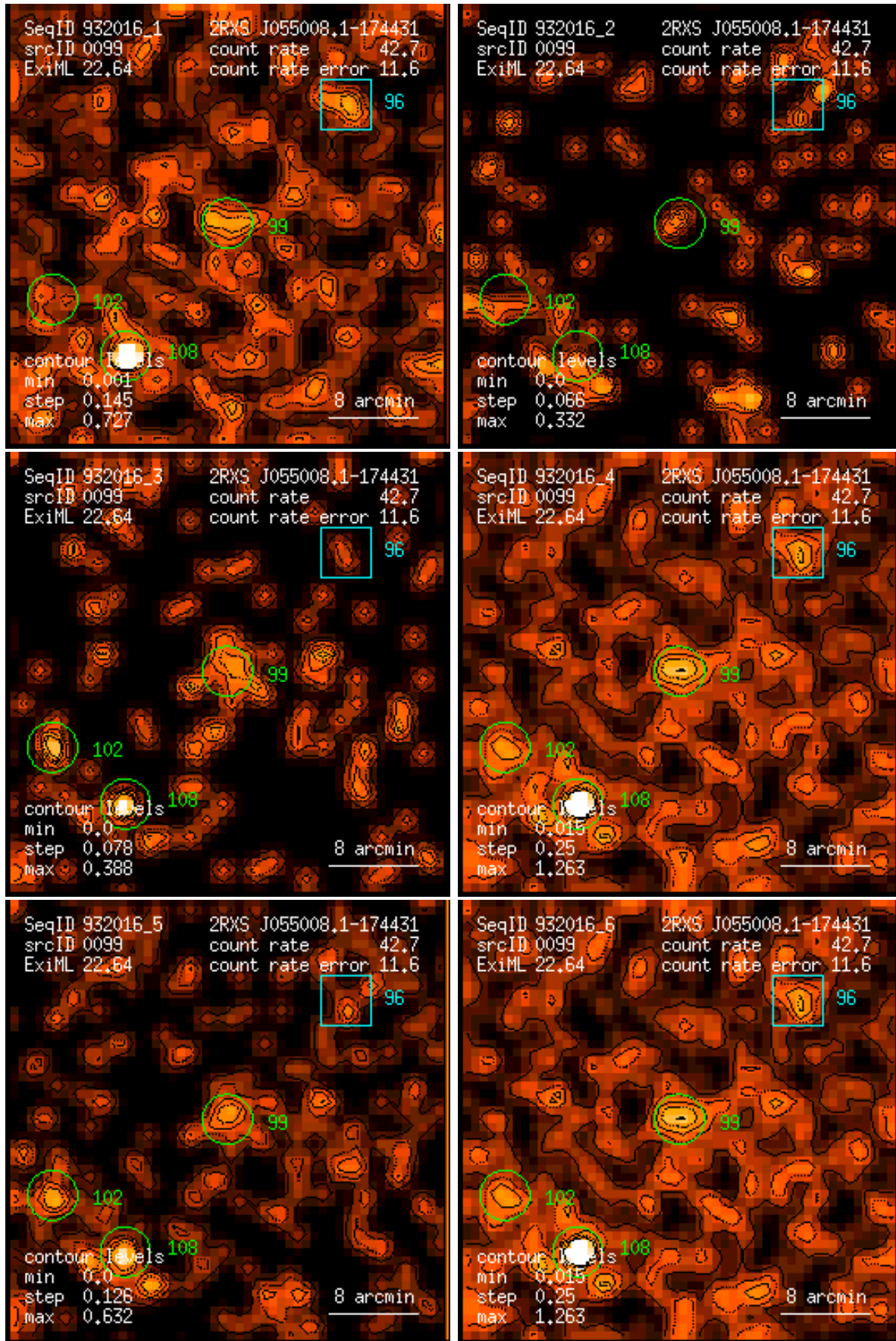
Figure 99: RASS 932016: detection 0099: band rate images, Gaussian filter: (1) PSPC channels 11 – 41, (2) 52 – 90, (3) 91 – 201, (4) 11 – 235, (5) 52 – 201, (6) 11 – 201. Broad band rates in counts/ks. Band rate contour levels in counts/ks/arcmin 2 .
