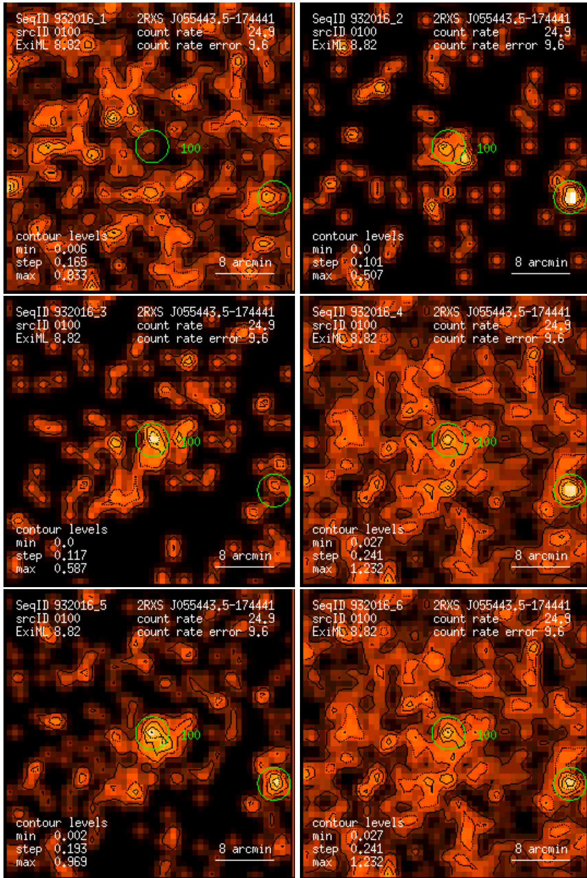
Figure 100: RASS 932016: detection 0100: band rate images, Gaussian filter: (1) PSPC channels 11 – 41, (2) 52 – 90, (3) 91 – 201, (4) 11 – 235, (5) 52 – 201, (6) 11 – 201. Broad band rates in counts/ks. Band rate contour levels in counts/ks/arcmin 2 .
