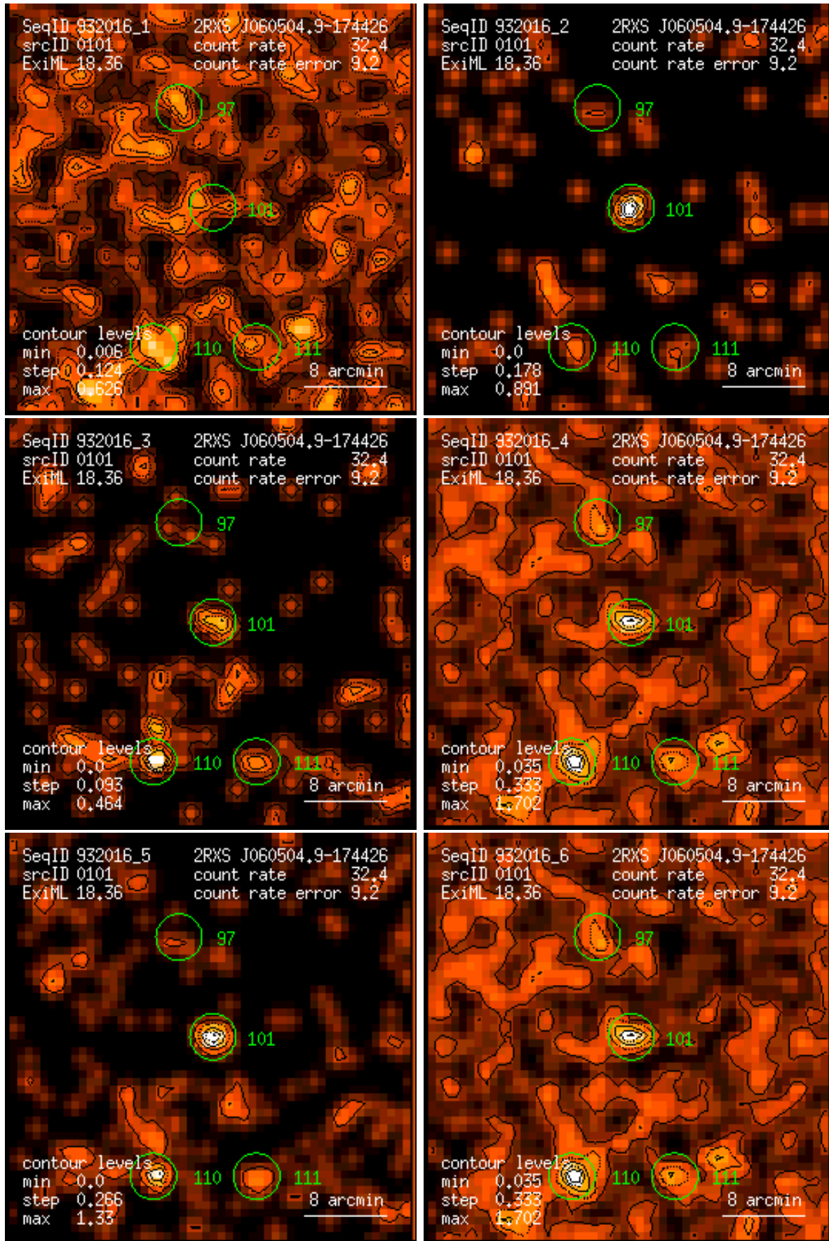
Figure 101: RASS 932016: detection 0101: band rate images, Gaussian filter: (1) PSPC channels 11 – 41, (2) 52 – 90, (3) 91 – 201, (4) 11 – 235, (5) 52 – 201, (6) 11 – 201. Broad band rates in counts/ks. Band rate contour levels in counts/ks/arcmin 2 .
