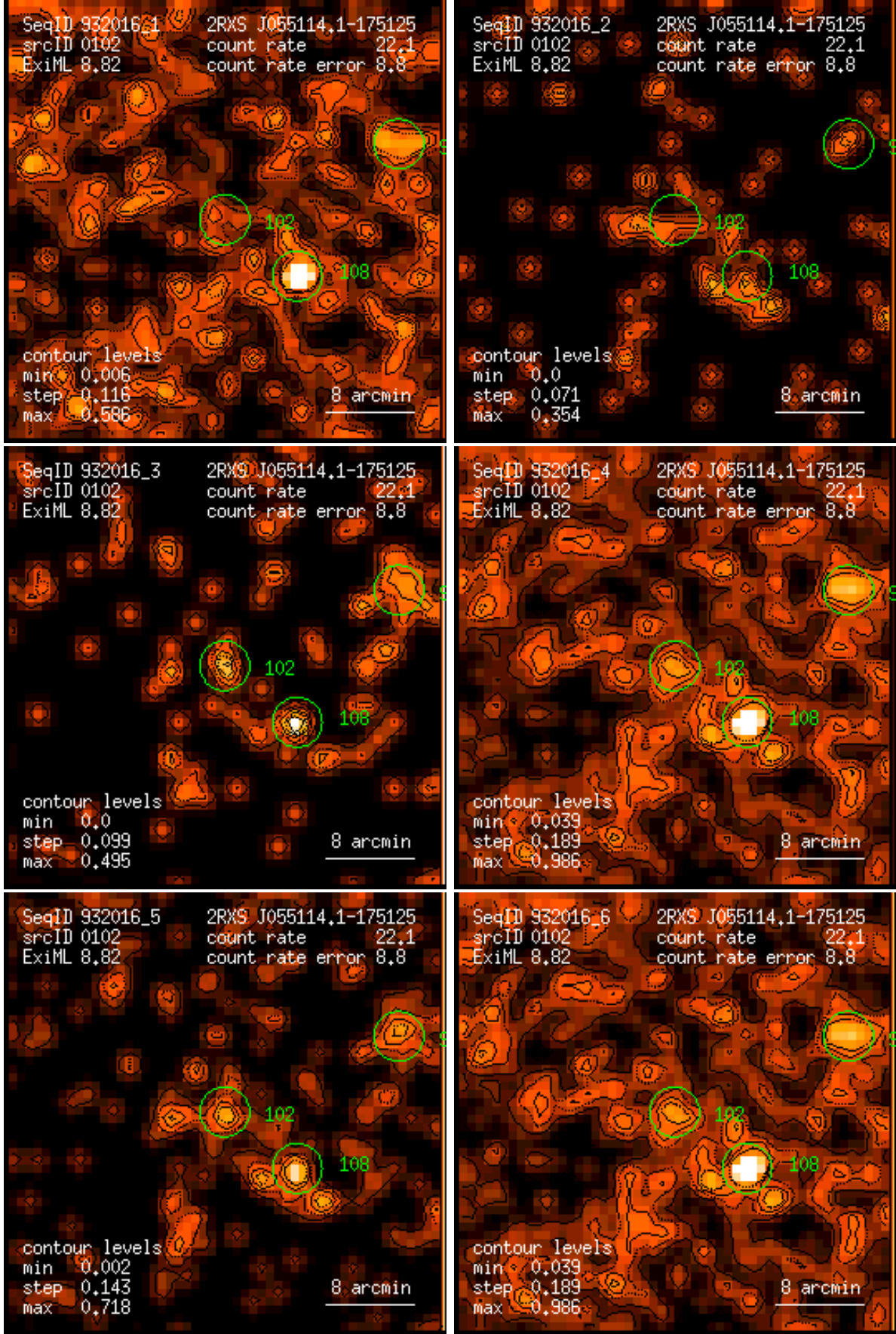
Figure 102: RASS 932016: detection 0102: band rate images, Gaussian filter: (1) PSPC channels 11 – 41, (2) 52 – 90, (3) 91 – 201, (4) 11 – 235, (5) 52 – 201, (6) 11 – 201. Broad band rates in counts/ks. Band rate contour levels in counts/ks/arcmin 2 .
