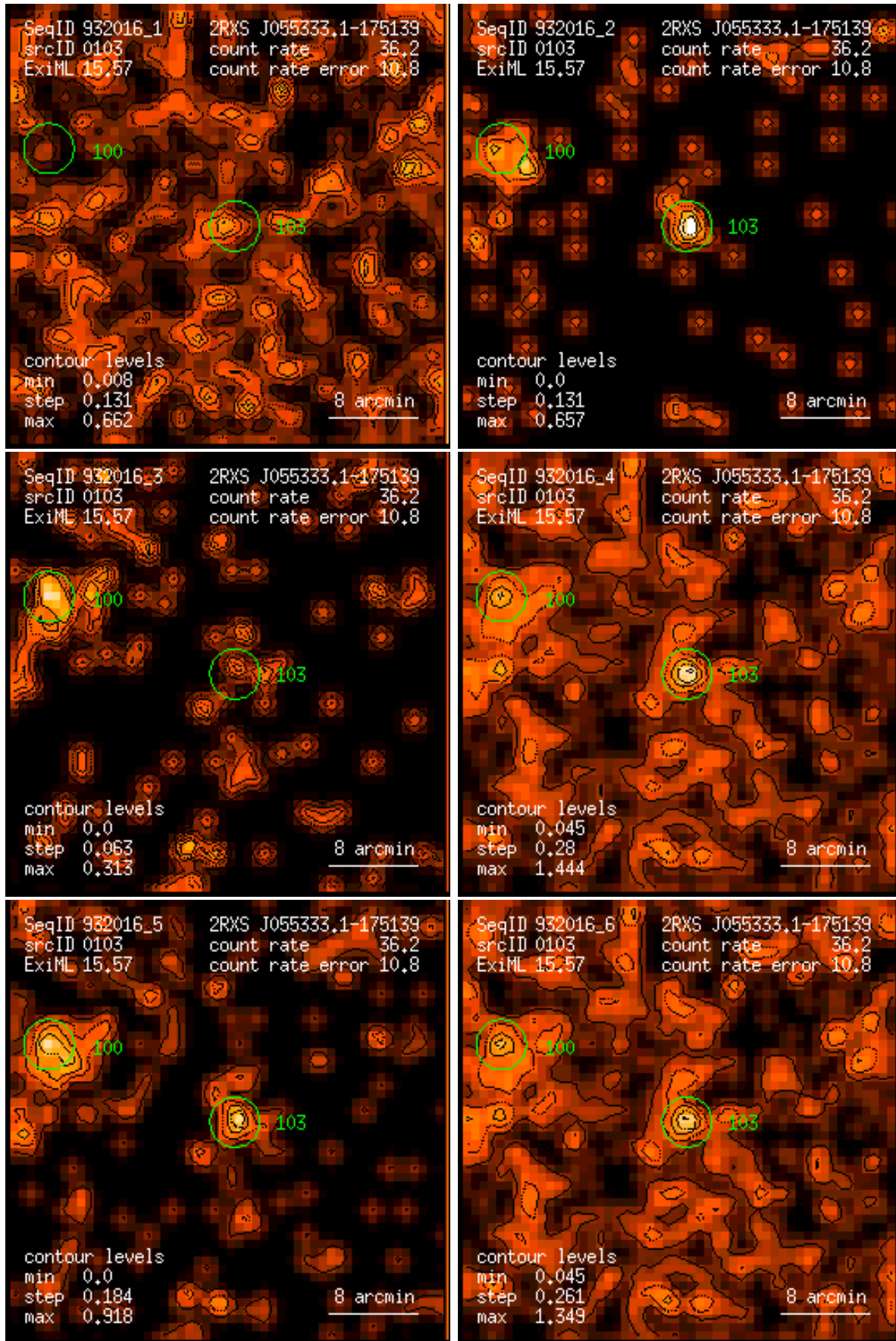
Figure 103: RASS 932016: detection 0103: band rate images, Gaussian filter: (1) PSPC channels 11 – 41, (2) 52 – 90, (3) 91 – 201, (4) 11 – 235, (5) 52 – 201, (6) 11 – 201. Broad band rates in counts/ks. Band rate contour levels in counts/ks/arcmin 2 .
