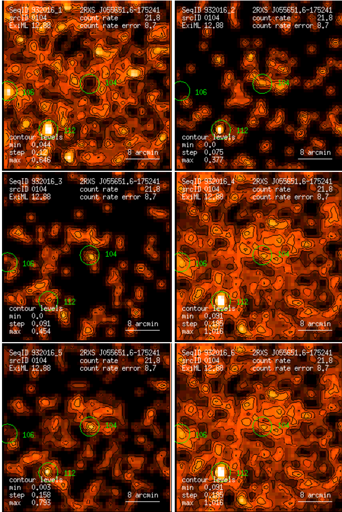
Figure 104: RASS 932016: detection 0104: band rate images, Gaussian filter: (1) PSPC channels 11 – 41, (2) 52 – 90, (3) 91 – 201, (4) 11 – 235, (5) 52 – 201, (6) 11 – 201. Broad band rates in counts/ks. Band rate contour levels in counts/ks/arcmin 2 .
