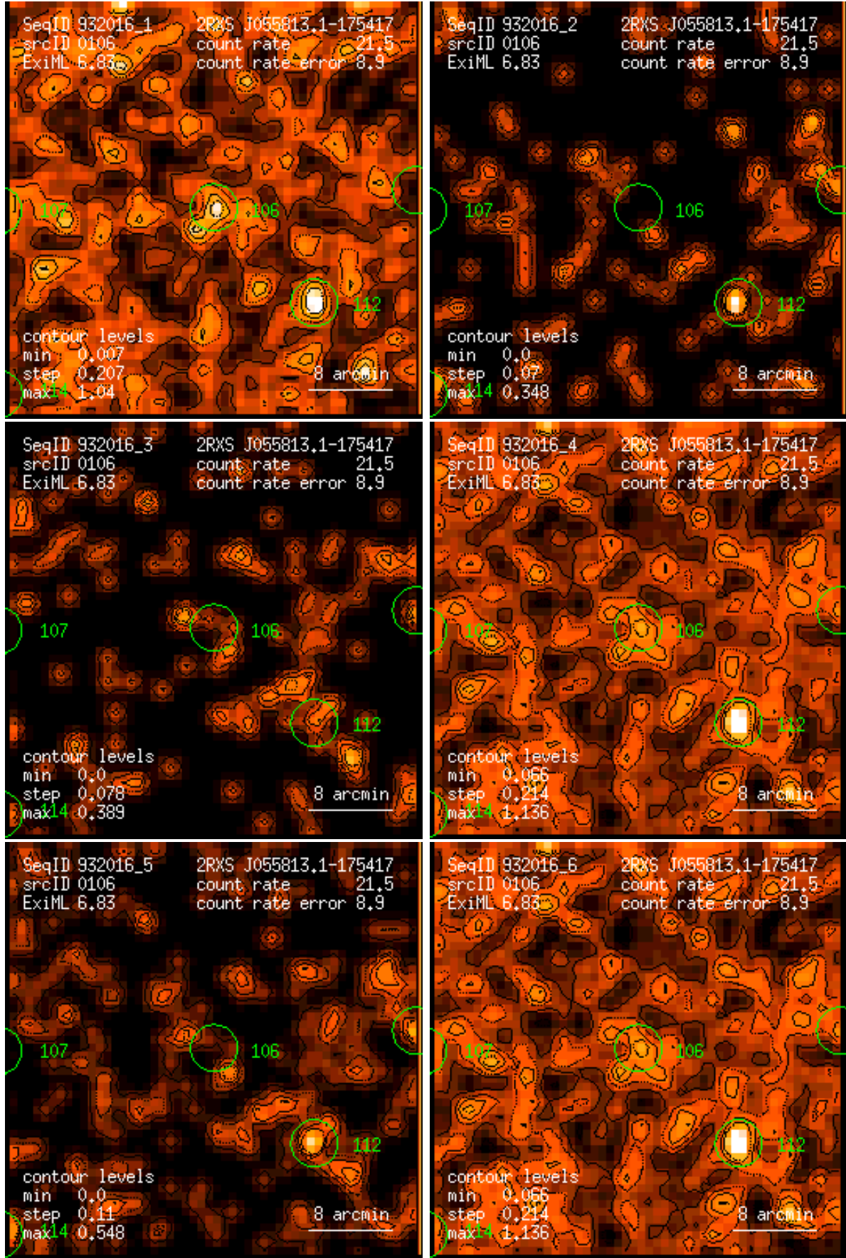
Figure 106: RASS 932016: detection 0106: band rate images, Gaussian filter: (1) PSPC channels 11 – 41, (2) 52 – 90, (3) 91 – 201, (4) 11 – 235, (5) 52 – 201, (6) 11 – 201. Broad band rates in counts/ks. Band rate contour levels in counts/ks/arcmin 2 .
