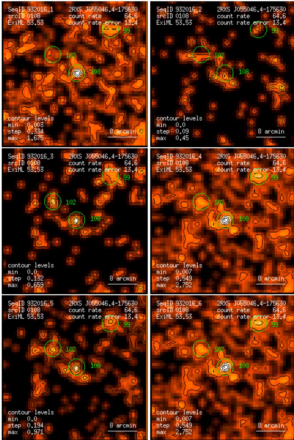
Figure 108: RASS 932016: detection 0108: band rate images, Gaussian filter: (1) PSPC channels 11 – 41, (2) 52 – 90, (3) 91 – 201, (4) 11 – 235, (5) 52 – 201, (6) 11 – 201. Broad band rates in counts/ks. Band rate contour levels in counts/ks/arcmin 2 .
