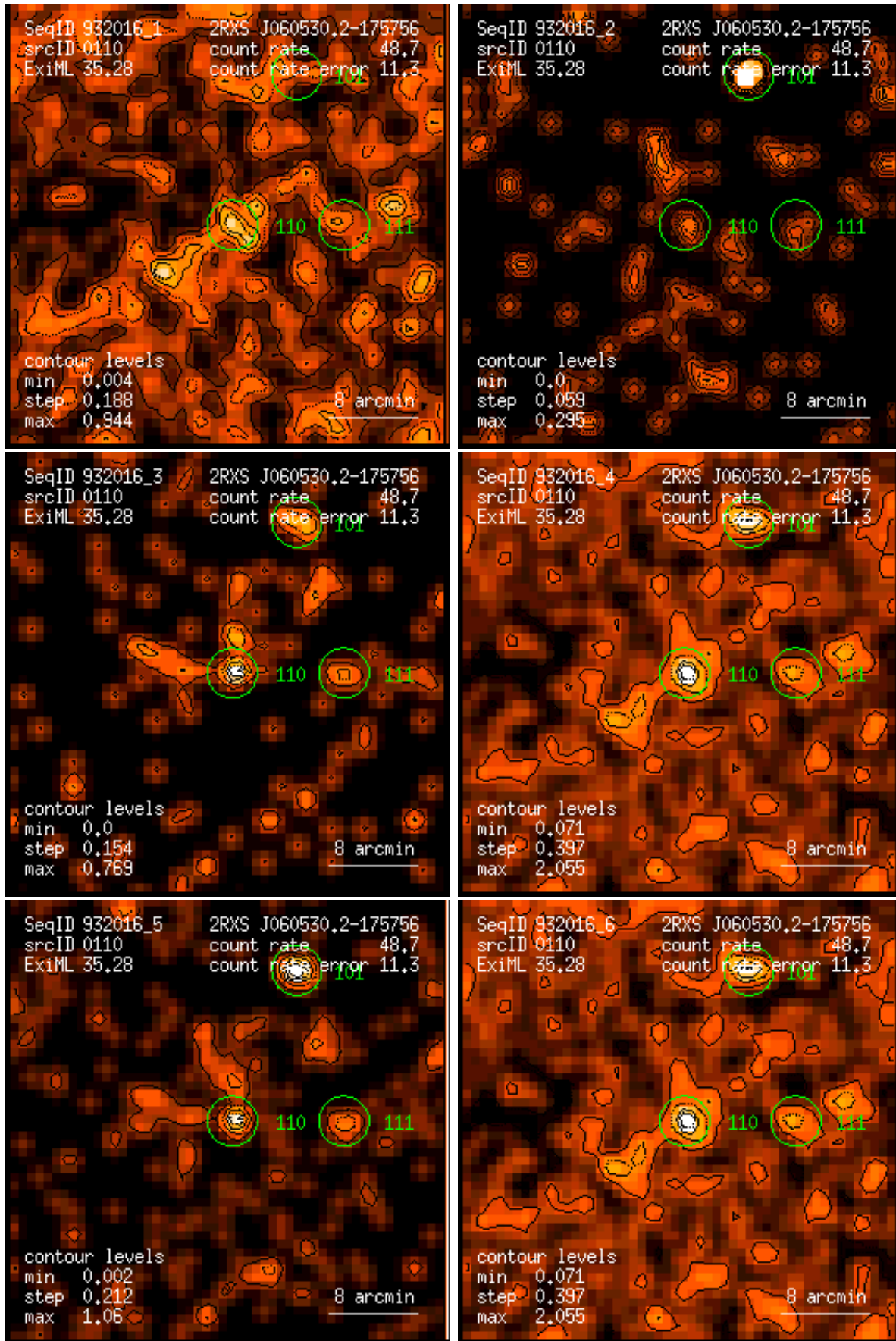
Figure 110: RASS 932016: detection 0110: band rate images, Gaussian filter: (1) PSPC channels 11 – 41, (2) 52 – 90, (3) 91 – 201, (4) 11 – 235, (5) 52 – 201, (6) 11 – 201. Broad band rates in counts/ks. Band rate contour levels in counts/ks/arcmin 2 .
