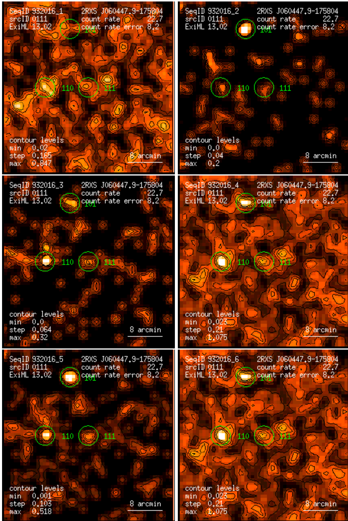
Figure 111: RASS 932016: detection 0111: band rate images, Gaussian filter: (1) PSPC channels 11 – 41, (2) 52 – 90, (3) 91 – 201, (4) 11 – 235, (5) 52 – 201, (6) 11 – 201. Broad band rates in counts/ks. Band rate contour levels in counts/ks/arcmin 2 .
