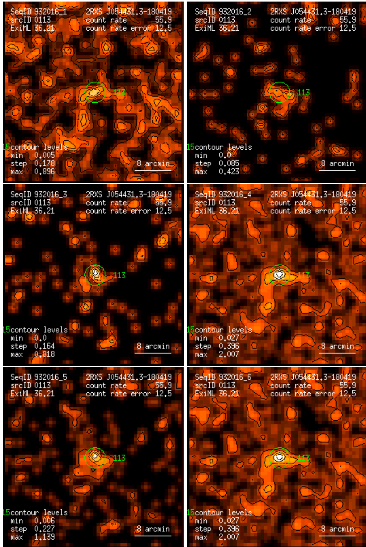
Figure 113: RASS 932016: detection 0113: band rate images, Gaussian filter: (1) PSPC channels 11 – 41, (2) 52 – 90, (3) 91 – 201, (4) 11 – 235, (5) 52 – 201, (6) 11 – 201. Broad band rates in counts/ks. Band rate contour levels in counts/ks/arcmin 2 .
