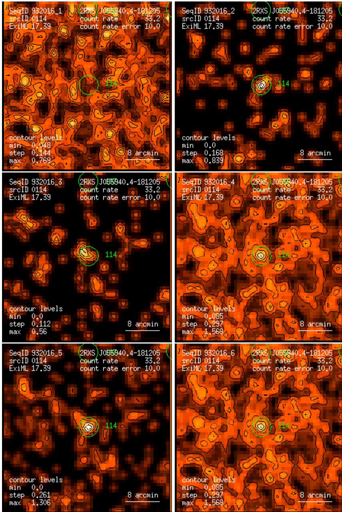
Figure 114: RASS 932016: detection 0114: band rate images, Gaussian filter: (1) PSPC channels 11 – 41, (2) 52 – 90, (3) 91 – 201, (4) 11 – 235, (5) 52 – 201, (6) 11 – 201. Broad band rates in counts/ks. Band rate contour levels in counts/ks/arcmin 2 .
