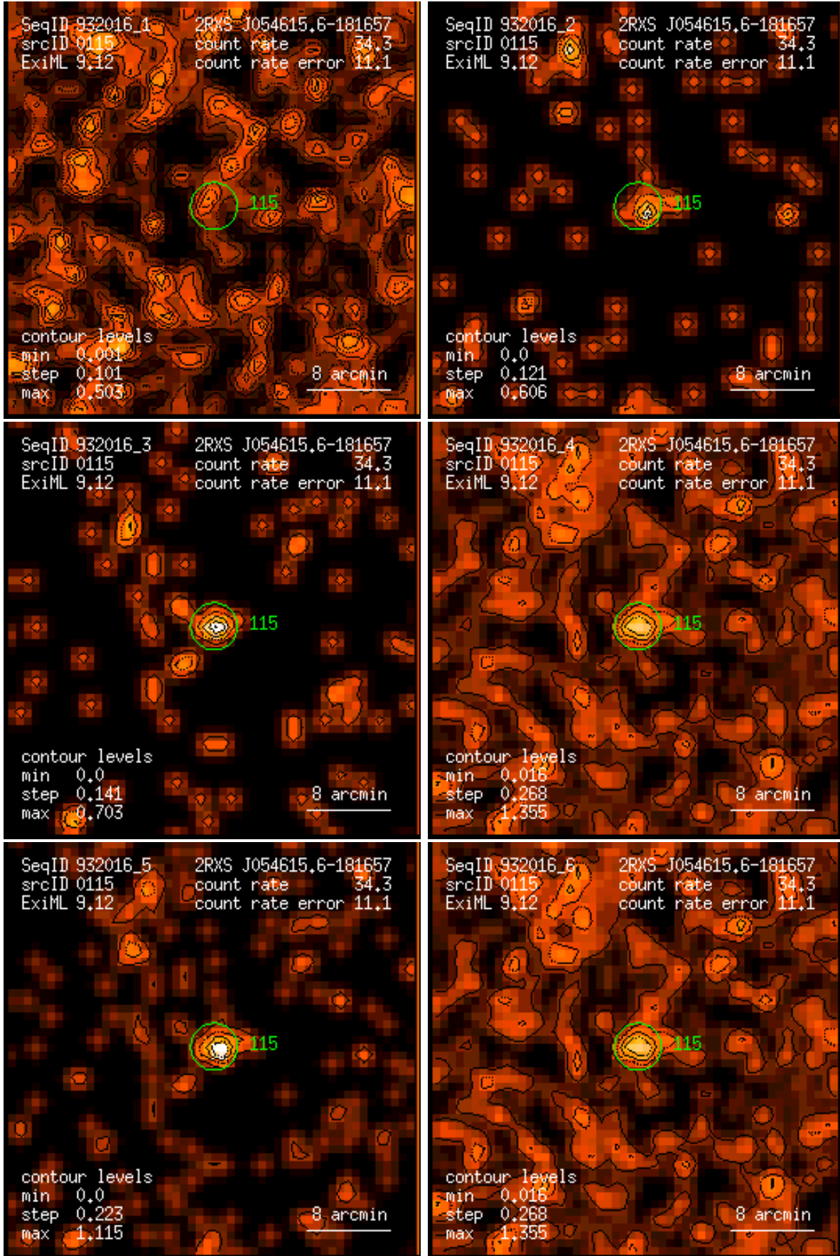
Figure 115: RASS 932016: detection 0115: band rate images, Gaussian filter: (1) PSPC channels 11 – 41, (2) 52 – 90, (3) 91 – 201, (4) 11 – 235, (5) 52 – 201, (6) 11 – 201. Broad band rates in counts/ks. Band rate contour levels in counts/ks/arcmin 2 .
