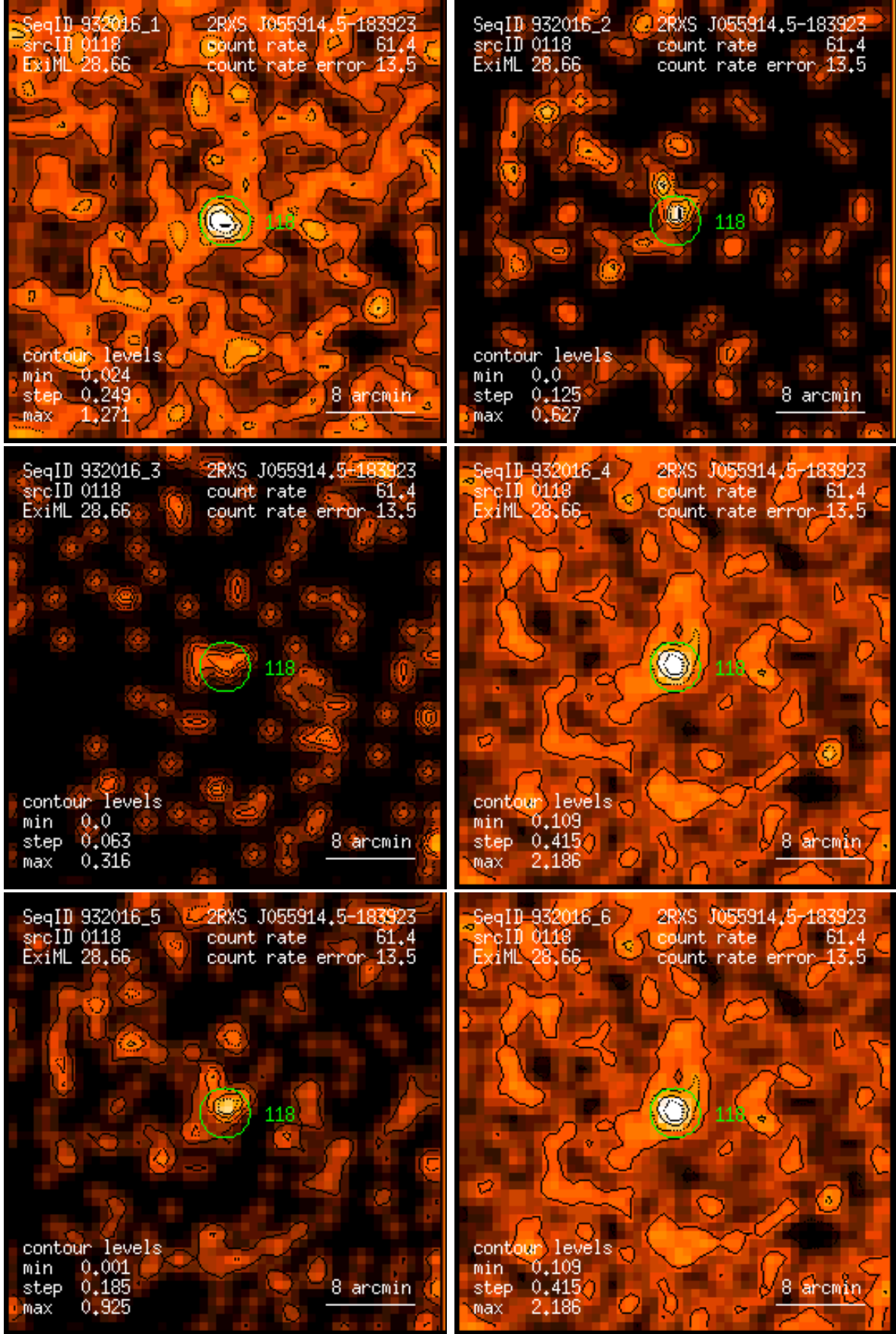
Figure 118: RASS 932016: detection 0118: band rate images, Gaussian filter: (1) PSPC channels 11 – 41, (2) 52 – 90, (3) 91 – 201, (4) 11 – 235, (5) 52 – 201, (6) 11 – 201. Broad band rates in counts/ks. Band rate contour levels in counts/ks/arcmin 2 .
