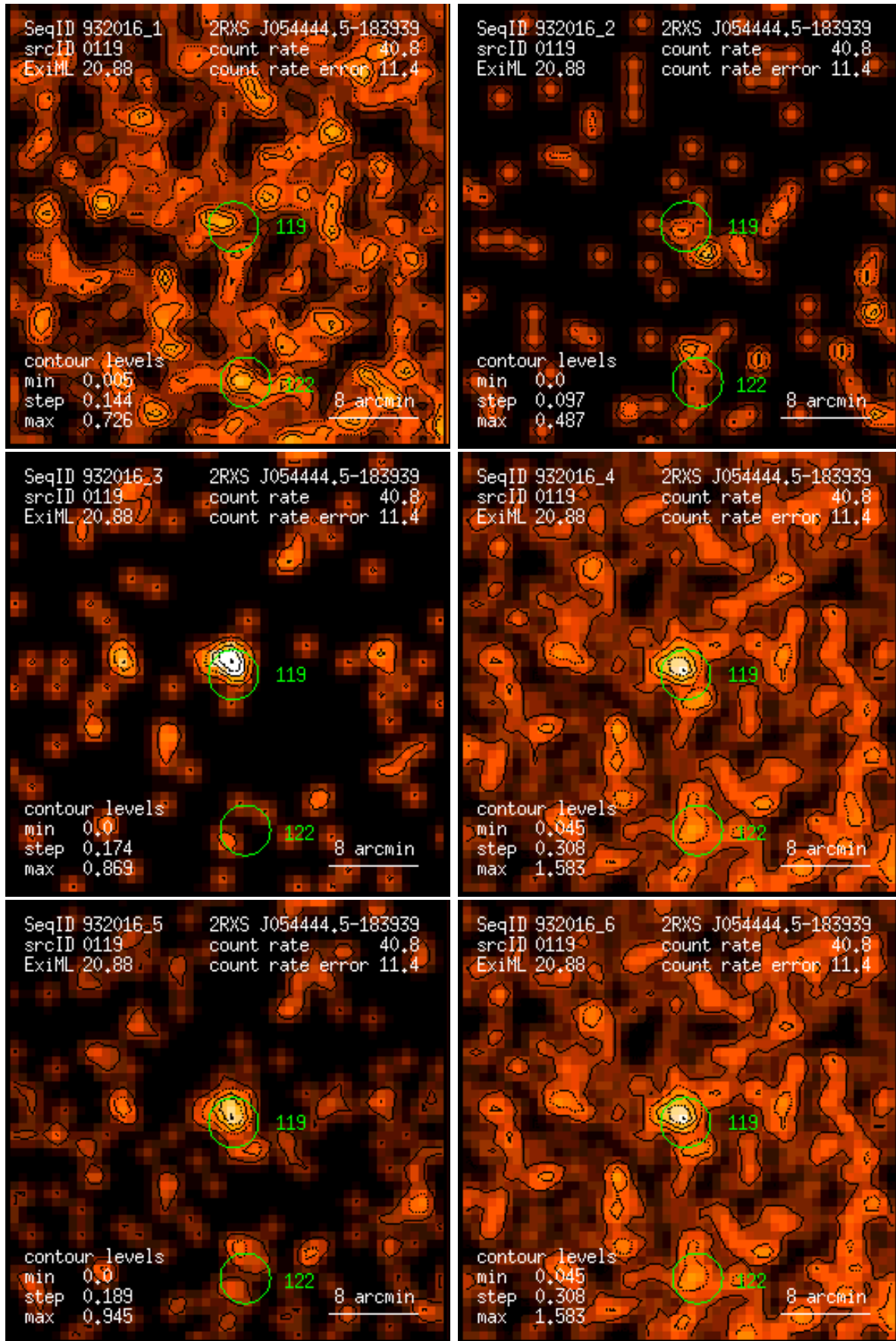
Figure 119: RASS 932016: detection 0119: band rate images, Gaussian filter: (1) PSPC channels 11 – 41, (2) 52 – 90, (3) 91 – 201, (4) 11 – 235, (5) 52 – 201, (6) 11 – 201. Broad band rates in counts/ks. Band rate contour levels in counts/ks/arcmin 2 .
