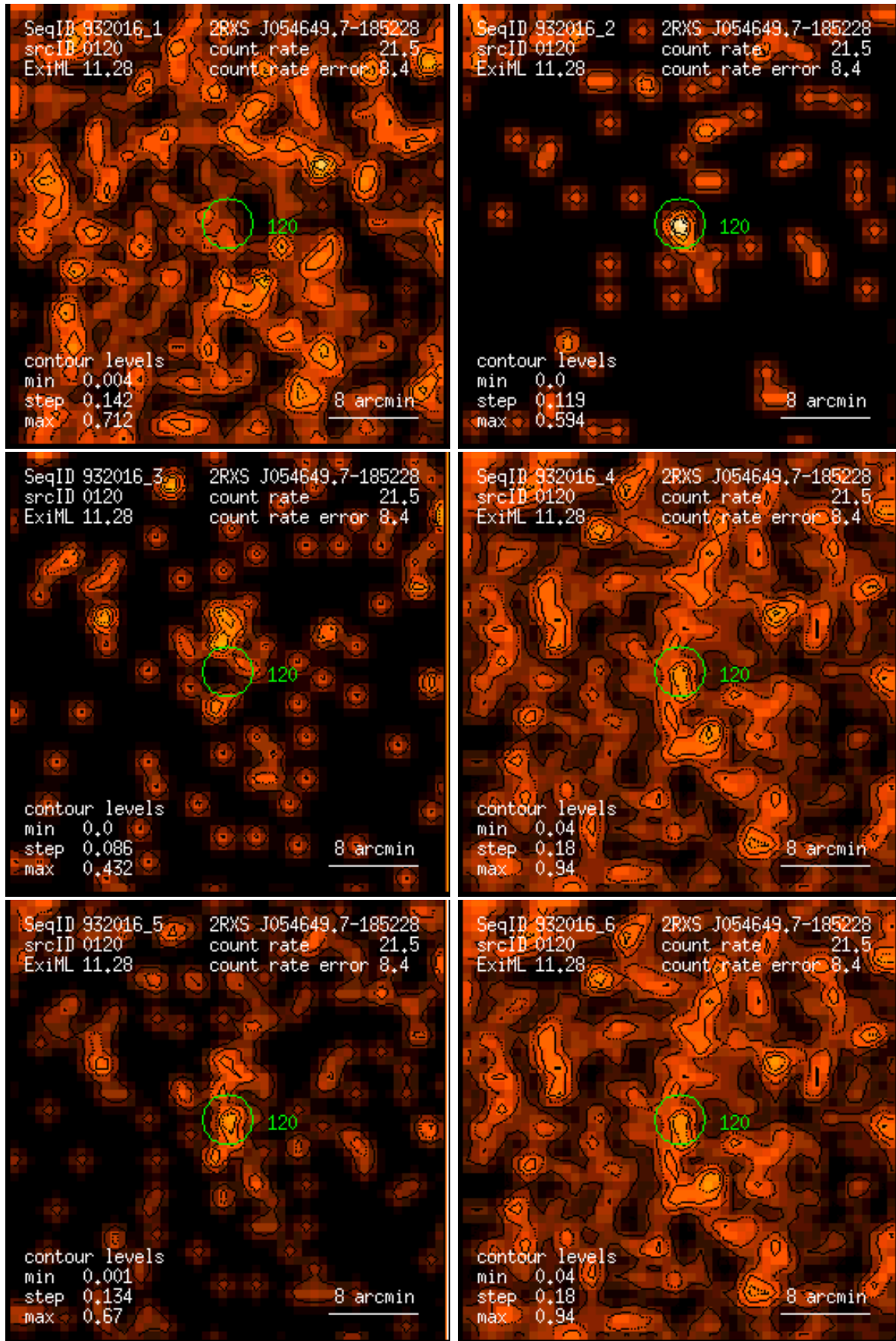
Figure 120: RASS 932016: detection 0120: band rate images, Gaussian filter: (1) PSPC channels 11 – 41, (2) 52 – 90, (3) 91 – 201, (4) 11 – 235, (5) 52 – 201, (6) 11 – 201. Broad band rates in counts/ks. Band rate contour levels in counts/ks/arcmin 2 .
