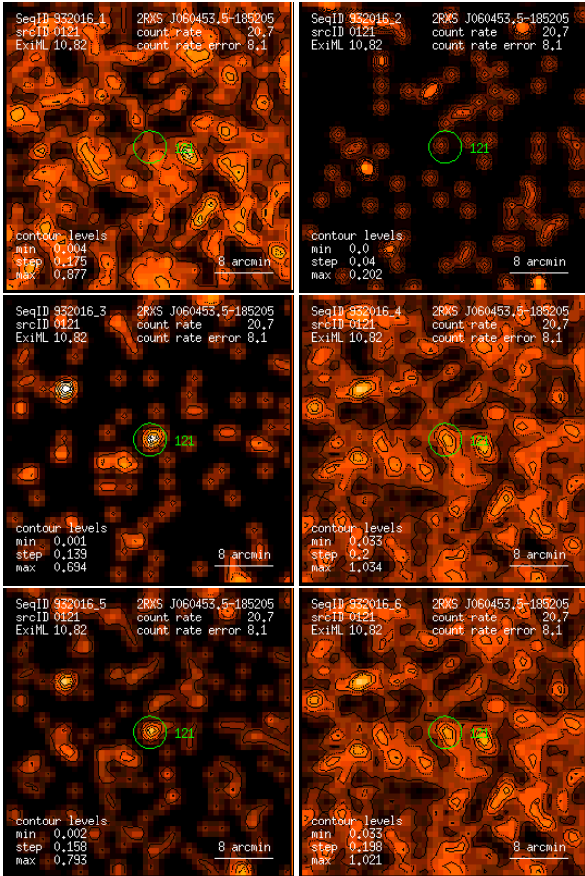
Figure 121: RASS 932016: detection 0121: band rate images, Gaussian filter: (1) PSPC channels 11 – 41, (2) 52 – 90, (3) 91 – 201, (4) 11 – 235, (5) 52 – 201, (6) 11 – 201. Broad band rates in counts/ks. Band rate contour levels in counts/ks/arcmin 2 .
