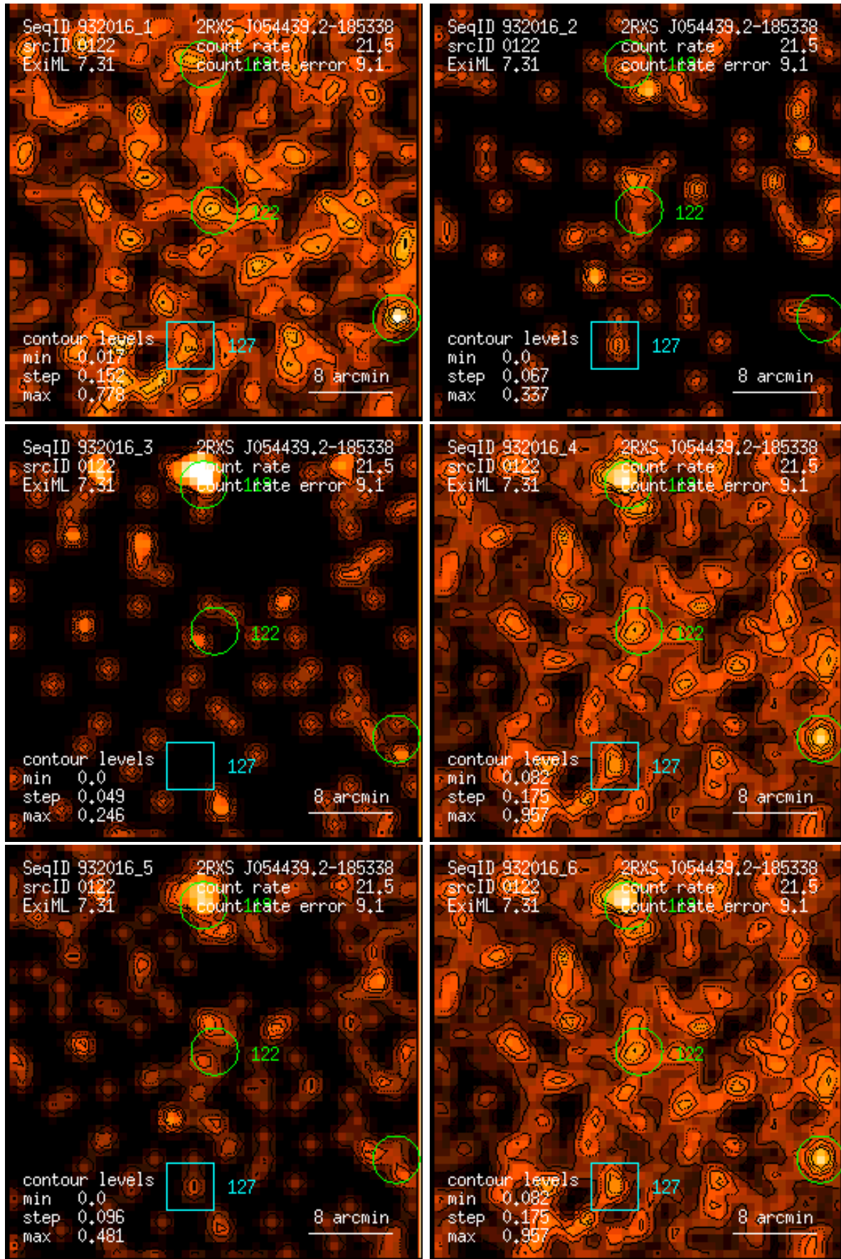
Figure 122: RASS 932016: detection 0122: band rate images, Gaussian filter: (1) PSPC channels 11 – 41, (2) 52 – 90, (3) 91 – 201, (4) 11 – 235, (5) 52 – 201, (6) 11 – 201. Broad band rates in counts/ks. Band rate contour levels in counts/ks/arcmin 2 .
