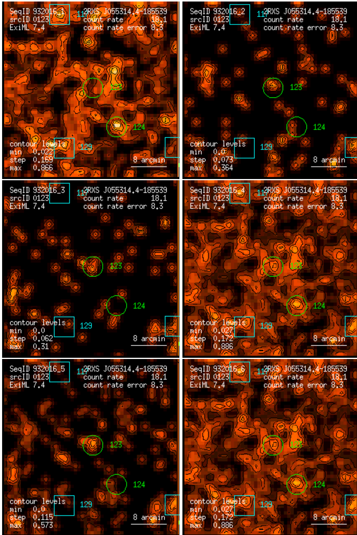
Figure 123: RASS 932016: detection 0123: band rate images, Gaussian filter: (1) PSPC channels 11 – 41, (2) 52 – 90, (3) 91 – 201, (4) 11 – 235, (5) 52 – 201, (6) 11 – 201. Broad band rates in counts/ks. Band rate contour levels in counts/ks/arcmin 2 .
