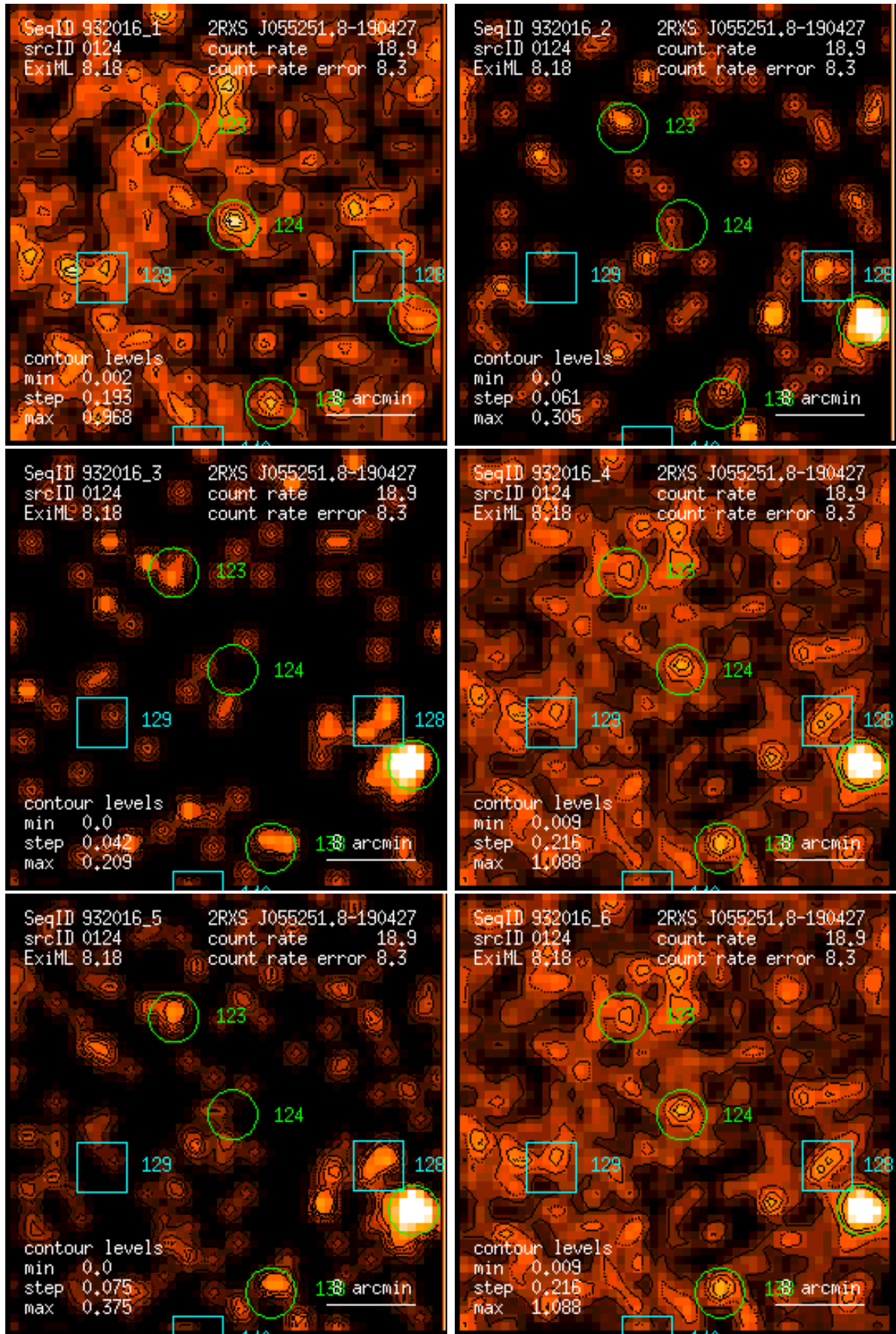
Figure 124: RASS 932016: detection 0124: band rate images, Gaussian filter: (1) PSPC channels 11 – 41, (2) 52 – 90, (3) 91 – 201, (4) 11 – 235, (5) 52 – 201, (6) 11 – 201. Broad band rates in counts/ks. Band rate contour levels in counts/ks/arcmin 2 .
