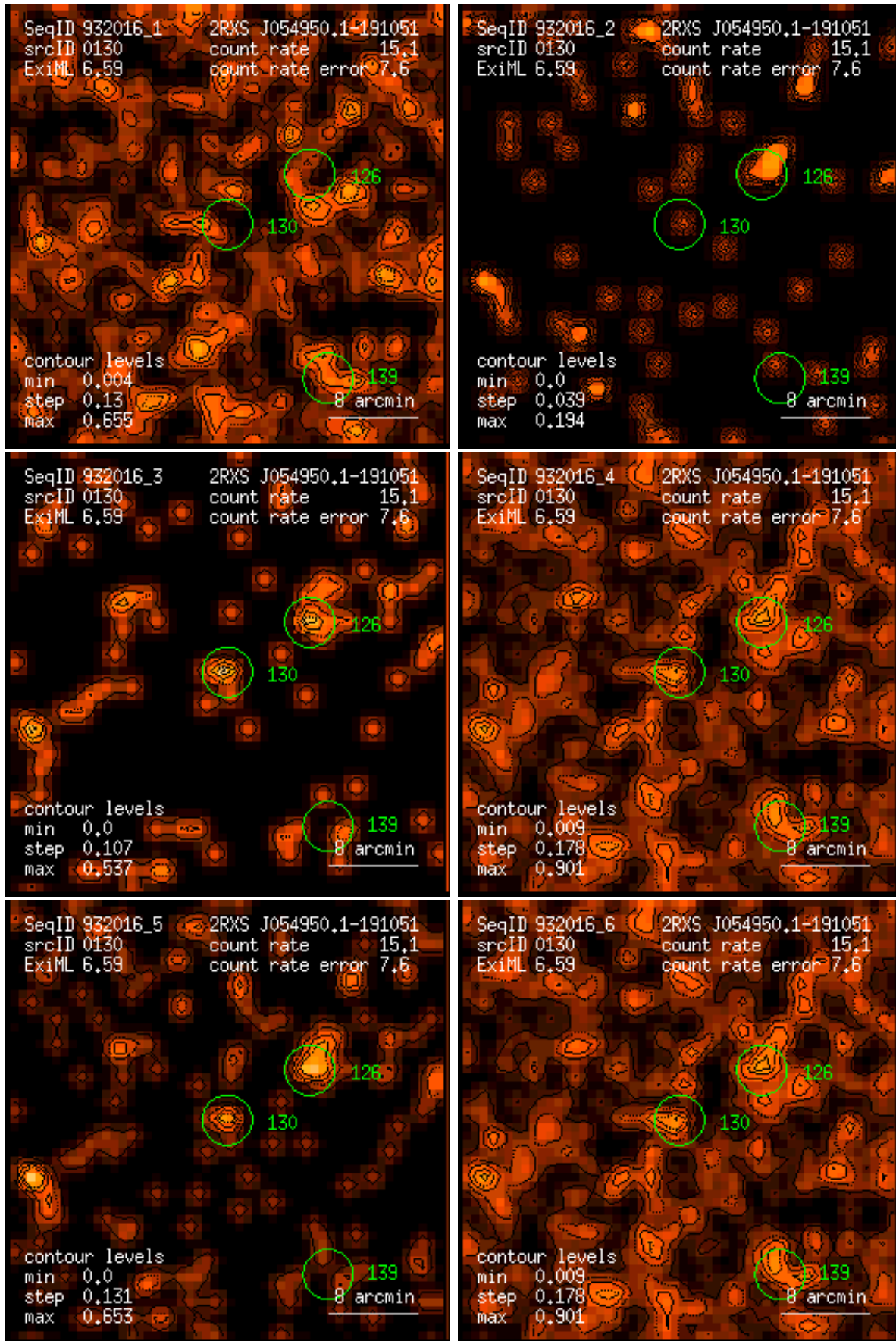
Figure 130: RASS 932016: detection 0130: band rate images, Gaussian filter: (1) PSPC channels 11 – 41, (2) 52 – 90, (3) 91 – 201, (4) 11 – 235, (5) 52 – 201, (6) 11 – 201. Broad band rates in counts/ks. Band rate contour levels in counts/ks/arcmin 2 .
