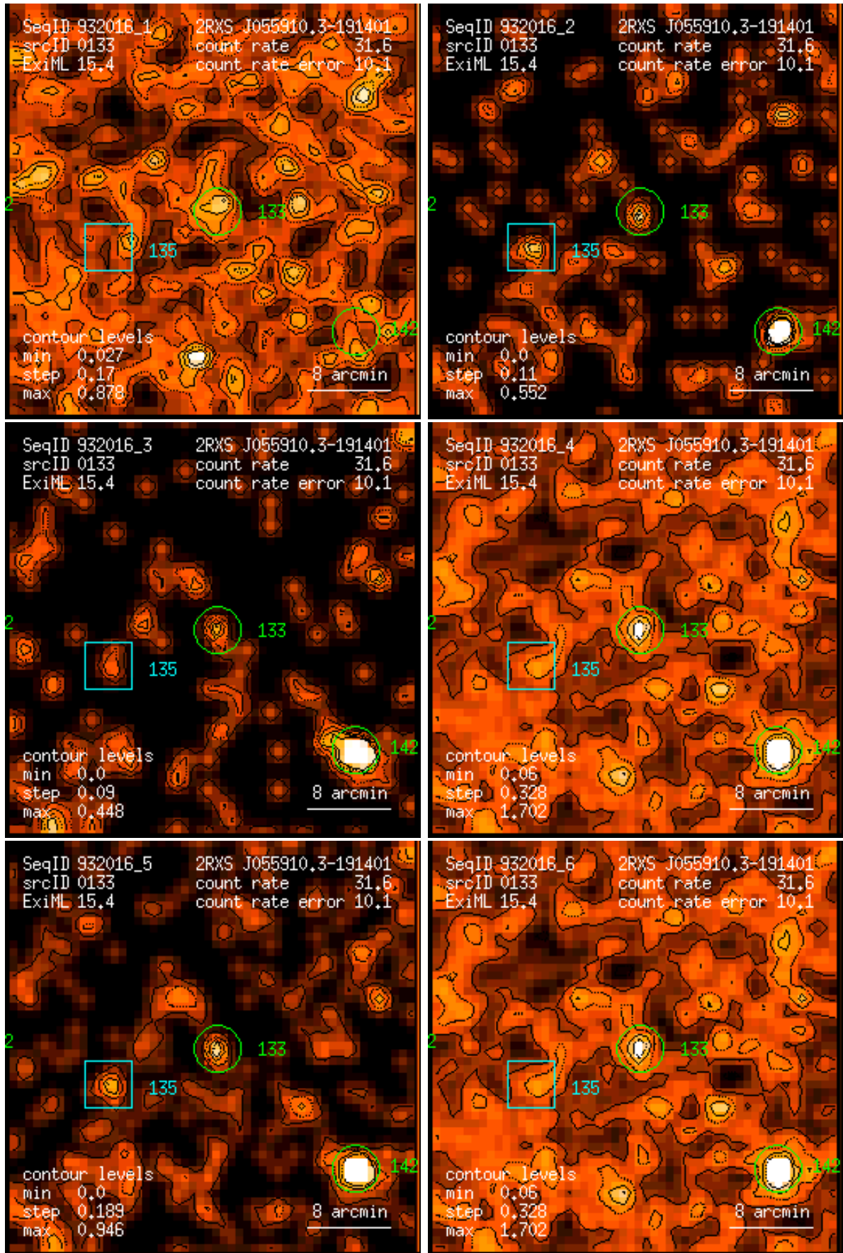
Figure 133: RASS 932016: detection 0133: band rate images, Gaussian filter: (1) PSPC channels 11 – 41, (2) 52 – 90, (3) 91 – 201, (4) 11 – 235, (5) 52 – 201, (6) 11 – 201. Broad band rates in counts/ks. Band rate contour levels in counts/ks/arcmin 2 .
