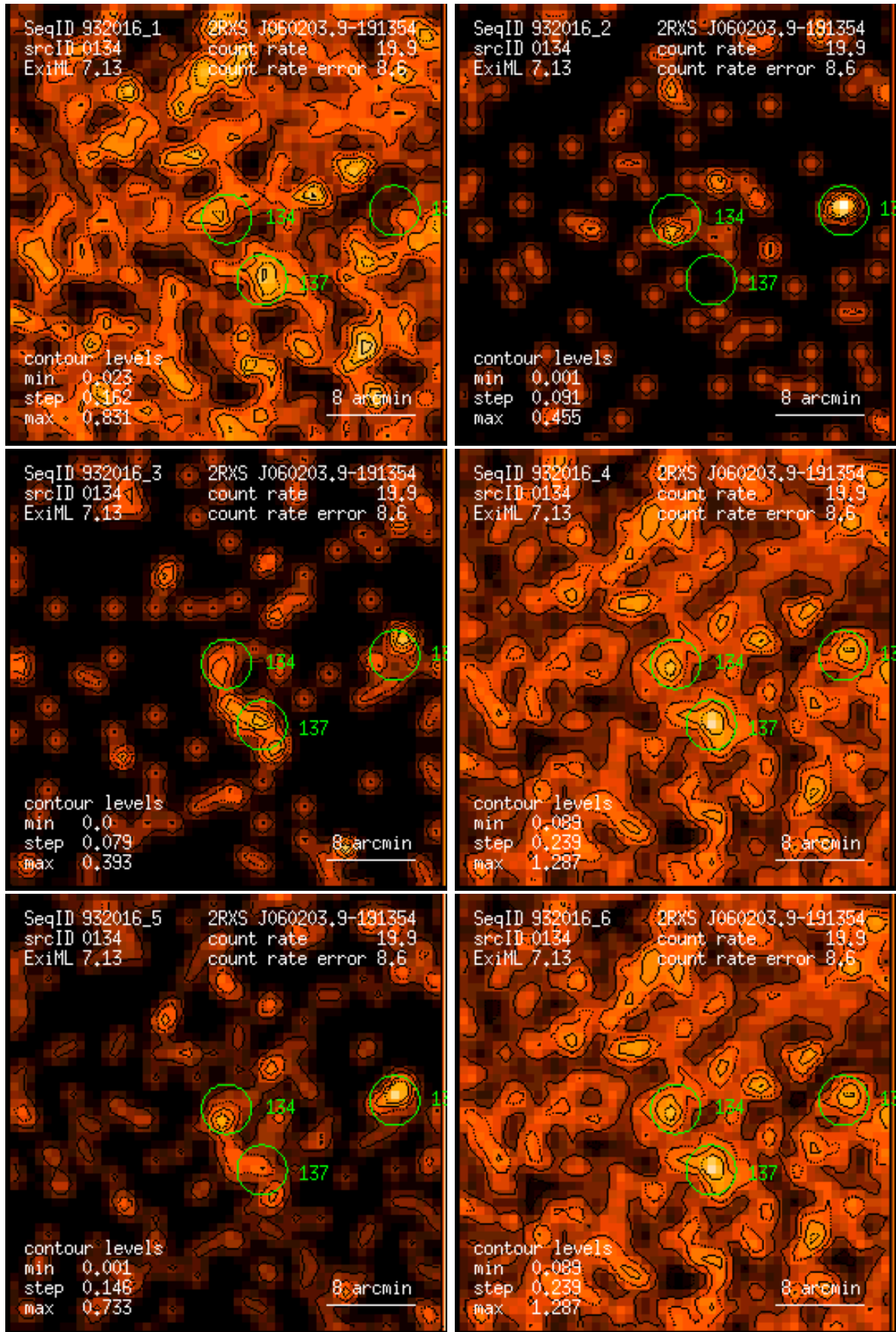
Figure 134: RASS 932016: detection 0134: band rate images, Gaussian filter: (1) PSPC channels 11 – 41, (2) 52 – 90, (3) 91 – 201, (4) 11 – 235, (5) 52 – 201, (6) 11 – 201. Broad band rates in counts/ks. Band rate contour levels in counts/ks/arcmin 2 .
