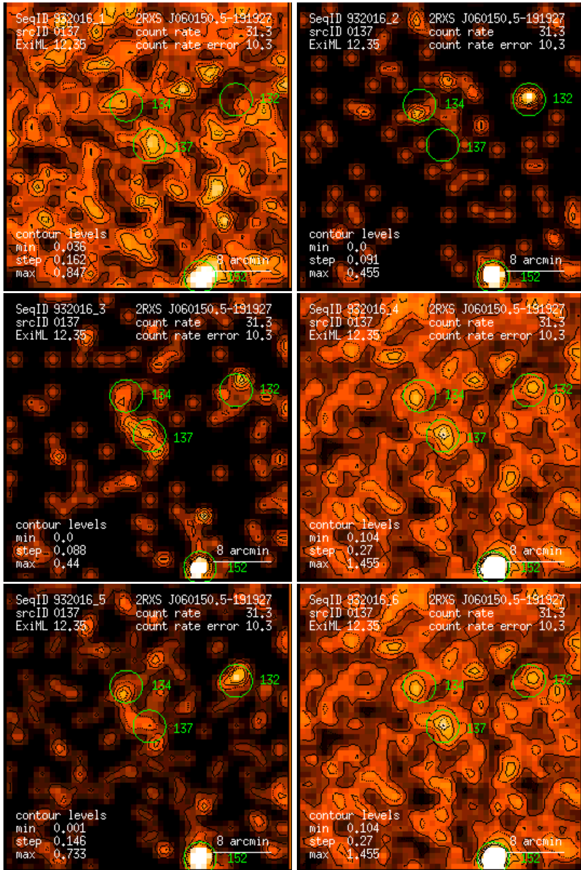
Figure 137: RASS 932016: detection 0137: band rate images, Gaussian filter: (1) PSPC channels 11 – 41, (2) 52 – 90, (3) 91 – 201, (4) 11 – 235, (5) 52 – 201, (6) 11 – 201. Broad band rates in counts/ks. Band rate contour levels in counts/ks/arcmin 2 .
