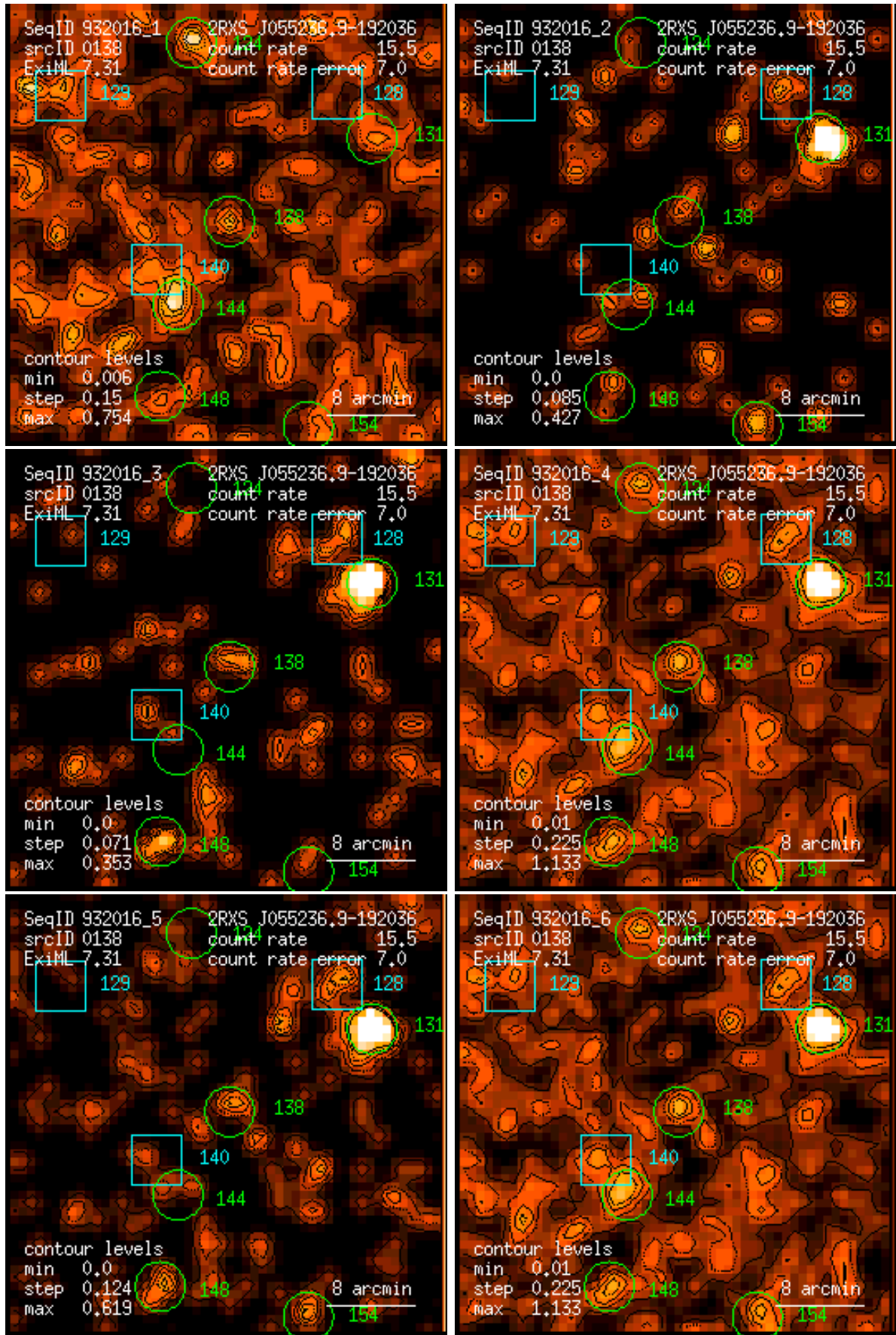
Figure 138: RASS 932016: detection 0138: band rate images, Gaussian filter: (1) PSPC channels 11 – 41, (2) 52 – 90, (3) 91 – 201, (4) 11 – 235, (5) 52 – 201, (6) 11 – 201. Broad band rates in counts/ks. Band rate contour levels in counts/ks/arcmin 2 .
