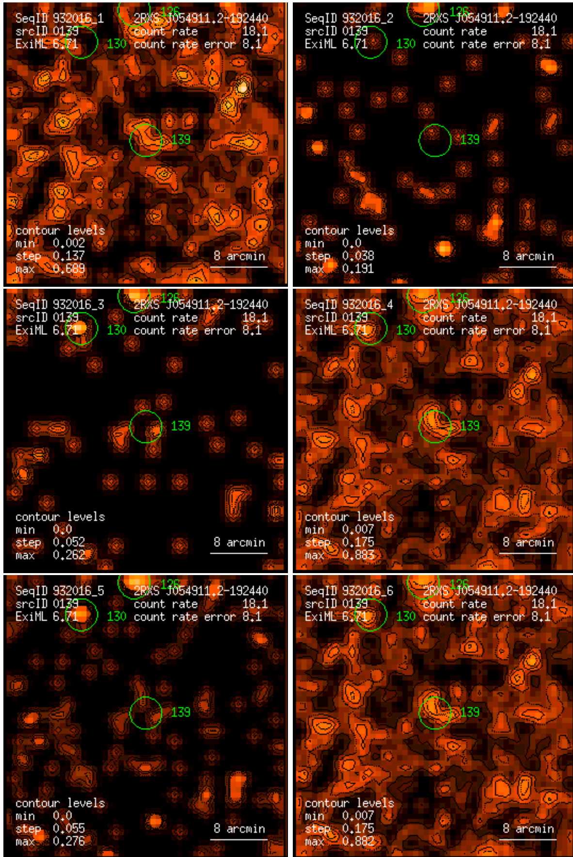
Figure 139: RASS 932016: detection 0139: band rate images, Gaussian filter: (1) PSPC channels 11 – 41, (2) 52 – 90, (3) 91 – 201, (4) 11 – 235, (5) 52 – 201, (6) 11 – 201. Broad band rates in counts/ks. Band rate contour levels in counts/ks/arcmin 2 .
