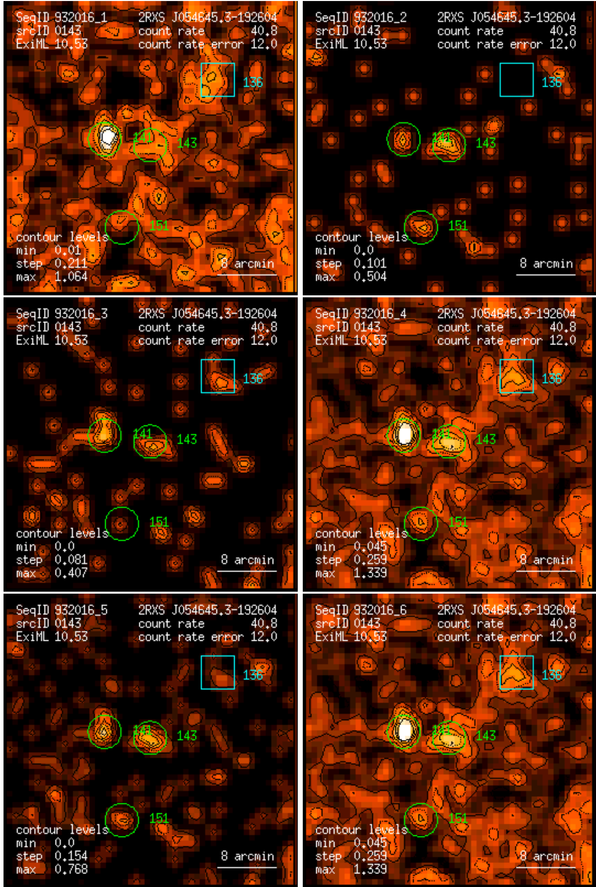
Figure 143: RASS 932016: detection 0143: band rate images, Gaussian filter: (1) PSPC channels 11 – 41, (2) 52 – 90, (3) 91 – 201, (4) 11 – 235, (5) 52 – 201, (6) 11 – 201. Broad band rates in counts/ks. Band rate contour levels in counts/ks/arcmin 2 .
