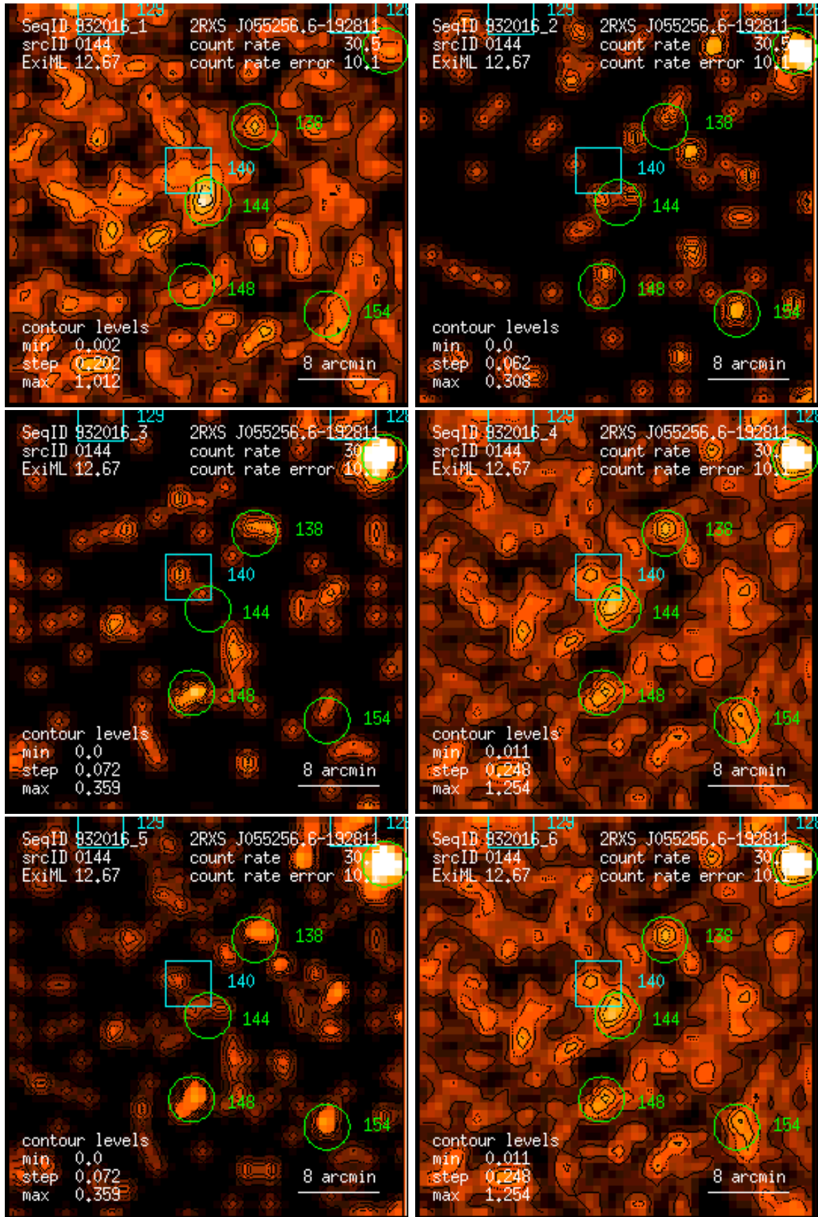
Figure 144: RASS 932016: detection 0144: band rate images, Gaussian filter: (1) PSPC channels 11 – 41, (2) 52 – 90, (3) 91 – 201, (4) 11 – 235, (5) 52 – 201, (6) 11 – 201. Broad band rates in counts/ks. Band rate contour levels in counts/ks/arcmin 2 .
