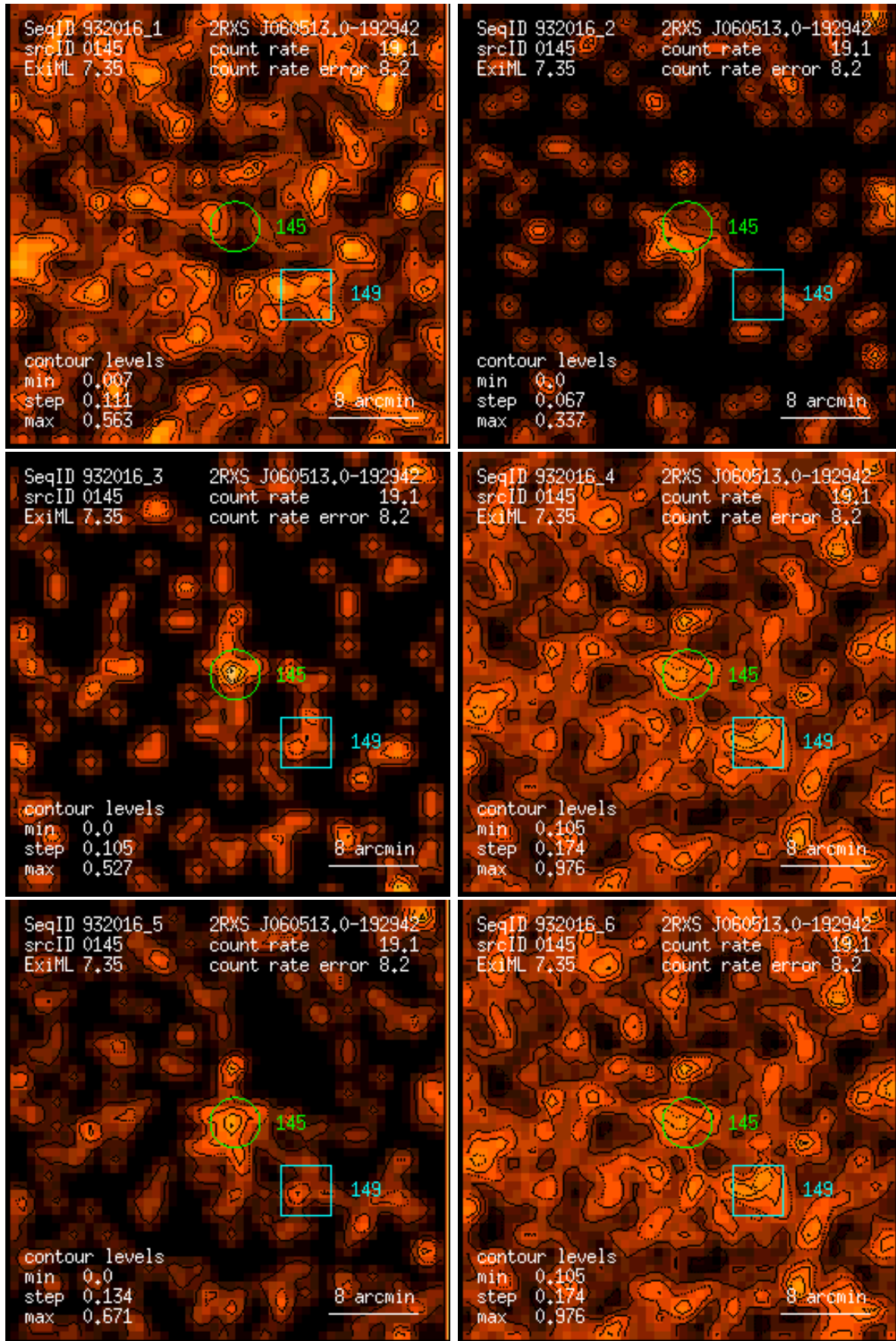
Figure 145: RASS 932016: detection 0145: band rate images, Gaussian filter: (1) PSPC channels 11 – 41, (2) 52 – 90, (3) 91 – 201, (4) 11 – 235, (5) 52 – 201, (6) 11 – 201. Broad band rates in counts/ks. Band rate contour levels in counts/ks/arcmin 2 .
