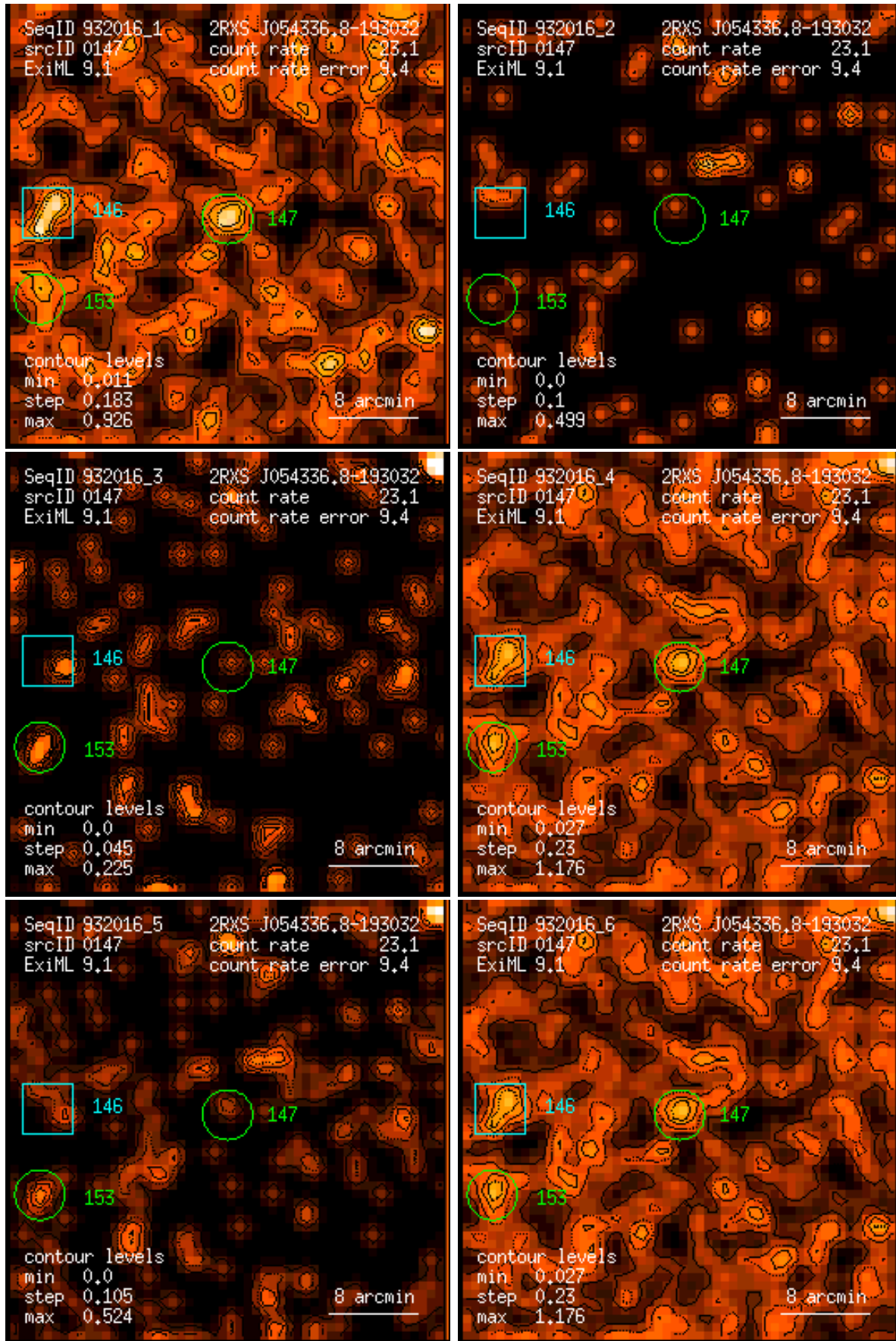
Figure 147: RASS 932016: detection 0147: band rate images, Gaussian filter: (1) PSPC channels 11 – 41, (2) 52 – 90, (3) 91 – 201, (4) 11 – 235, (5) 52 – 201, (6) 11 – 201. Broad band rates in counts/ks. Band rate contour levels in counts/ks/arcmin 2 .
