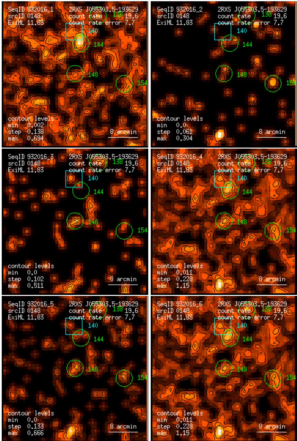
Figure 148: RASS 932016: detection 0148: band rate images, Gaussian filter: (1) PSPC channels 11 – 41, (2) 52 – 90, (3) 91 – 201, (4) 11 – 235, (5) 52 – 201, (6) 11 – 201. Broad band rates in counts/ks. Band rate contour levels in counts/ks/arcmin 2 .
