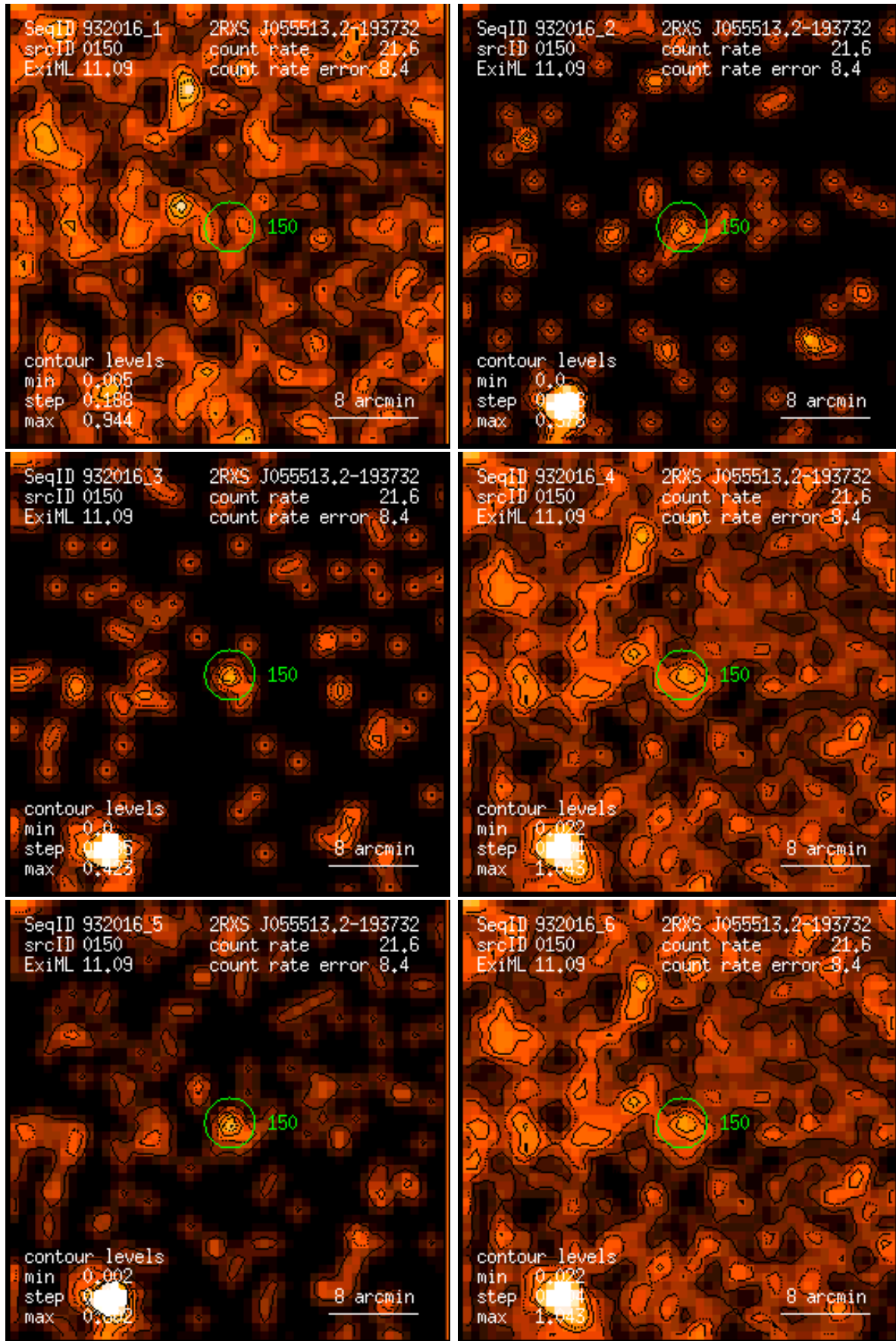
Figure 150: RASS 932016: detection 0150: band rate images, Gaussian filter: (1) PSPC channels 11 – 41, (2) 52 – 90, (3) 91 – 201, (4) 11 – 235, (5) 52 – 201, (6) 11 – 201. Broad band rates in counts/ks. Band rate contour levels in counts/ks/arcmin 2 .
