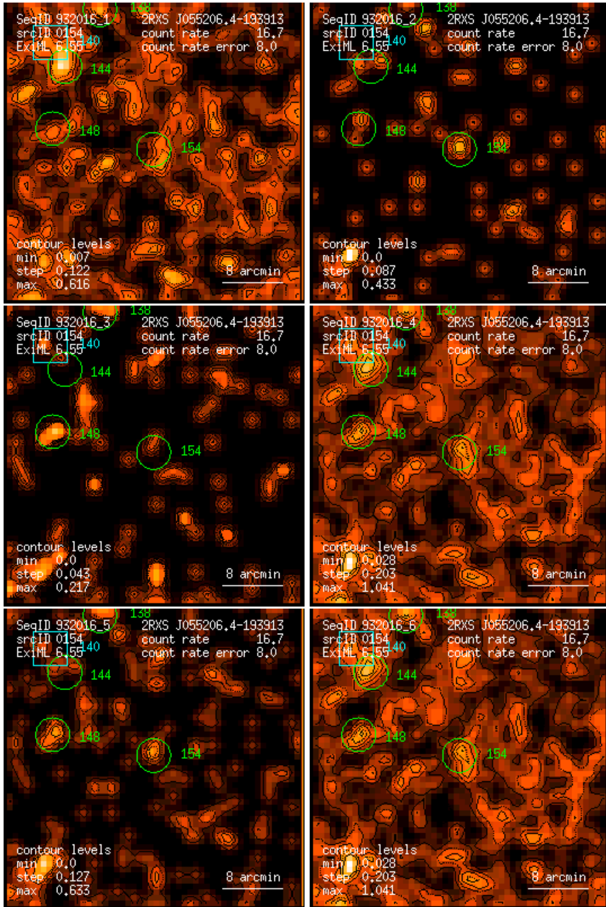
Figure 154: RASS 932016: detection 0154: band rate images, Gaussian filter: (1) PSPC channels 11 – 41, (2) 52 – 90, (3) 91 – 201, (4) 11 – 235, (5) 52 – 201, (6) 11 – 201. Broad band rates in counts/ks. Band rate contour levels in counts/ks/arcmin 2 .
