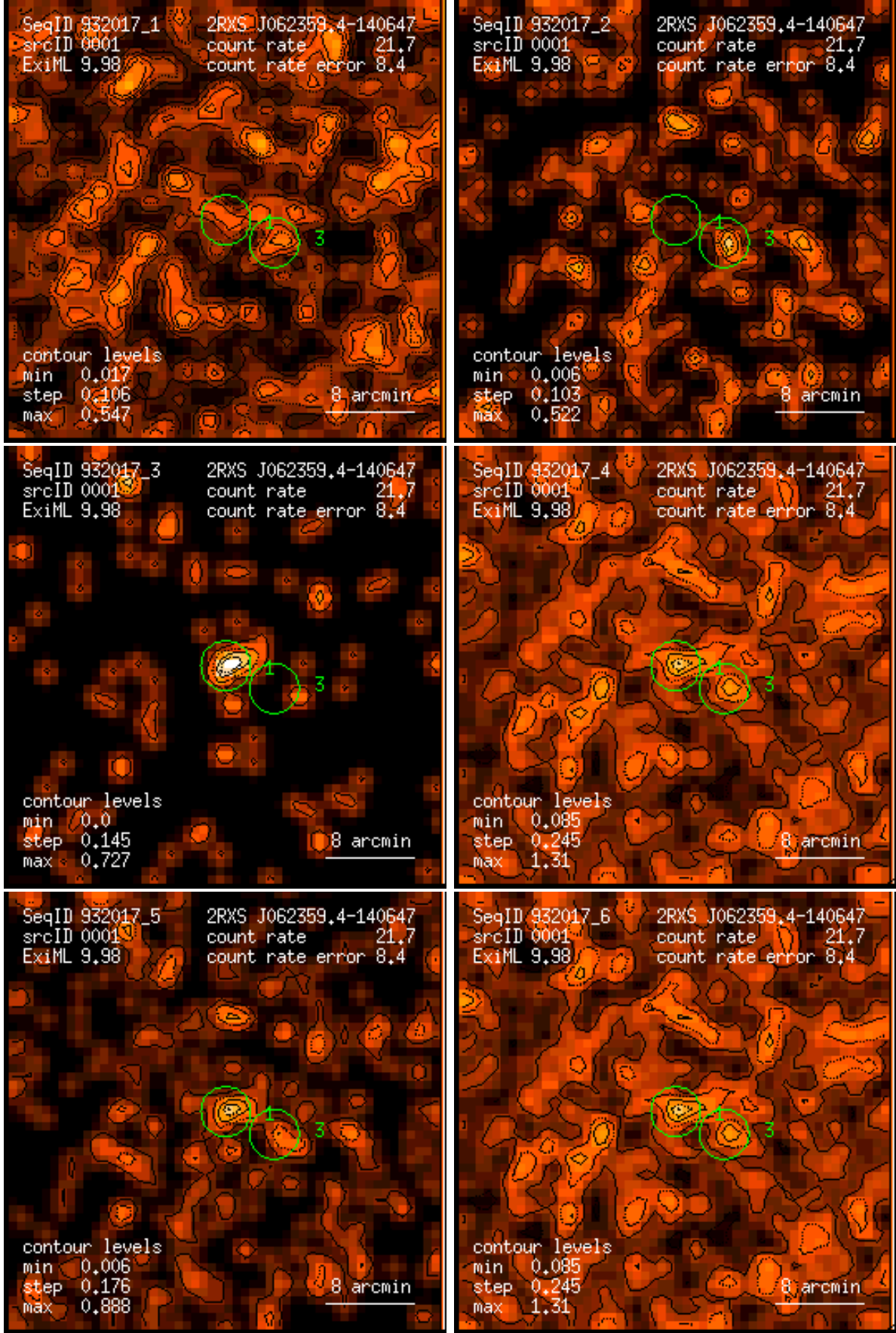
Figure 1: RASS 932017: detection 0001: band rate images, Gaussian filter: (1) PSPC channels 11 – 41, (2) 52 – 90, (3) 91 – 201, (4) 11 – 235, (5) 52 – 201, (6) 11 – 201. Broad band rates in counts/ks. Band rate contour levels in counts/ks/arcmin 2 .
