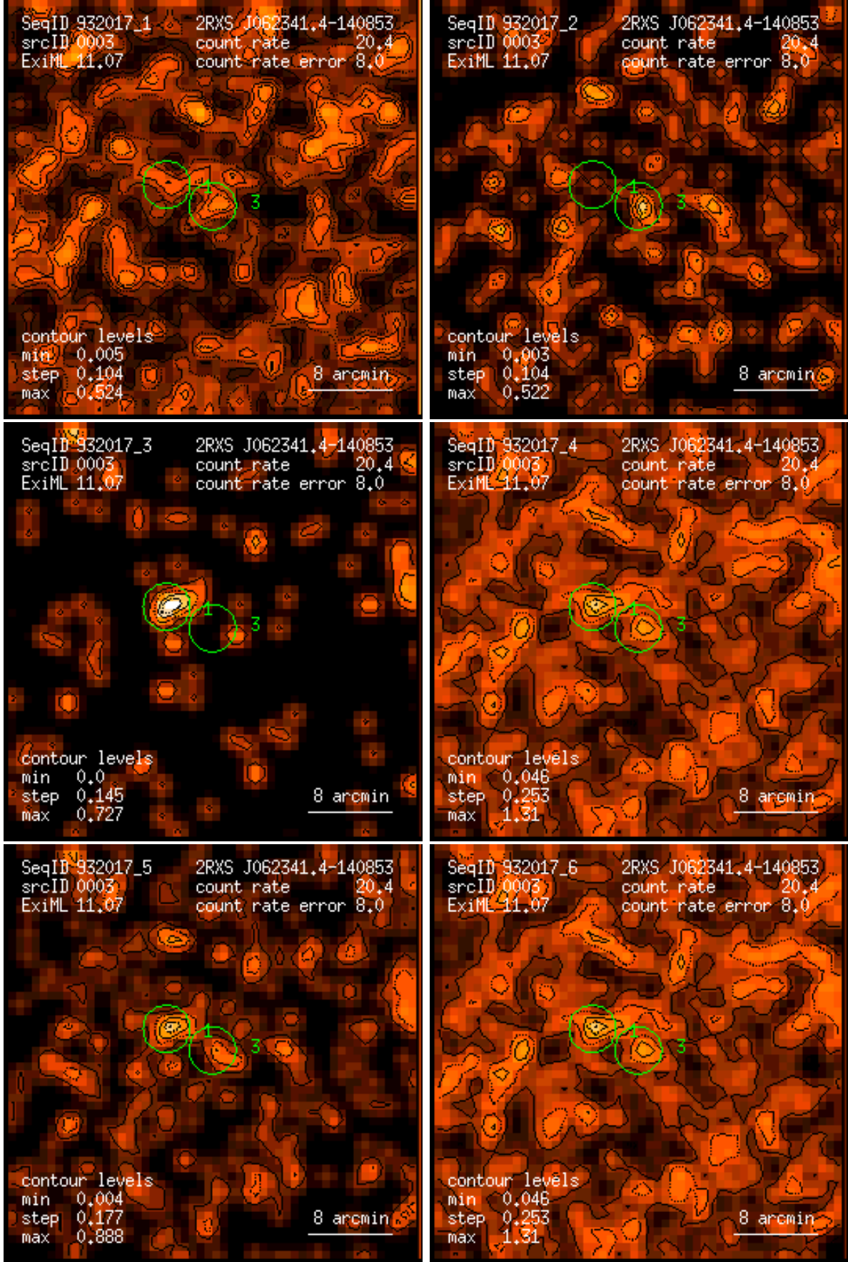
Figure 3: RASS 932017: detection 0003: band rate images, Gaussian filter: (1) PSPC channels 11 – 41, (2) 52 – 90, (3) 91 – 201, (4) 11 – 235, (5) 52 – 201, (6) 11 – 201. Broad band rates in counts/ks. Band rate contour levels in counts/ks/arcmin 2 .
