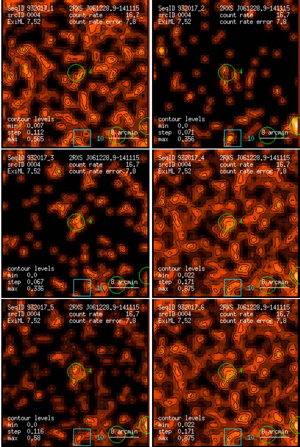
Figure 4: RASS 932017: detection 0004: band rate images, Gaussian filter: (1) PSPC channels 11 – 41, (2) 52 – 90, (3) 91 – 201, (4) 11 – 235, (5) 52 – 201, (6) 11 – 201. Broad band rates in counts/ks. Band rate contour levels in counts/ks/arcmin 2 .
