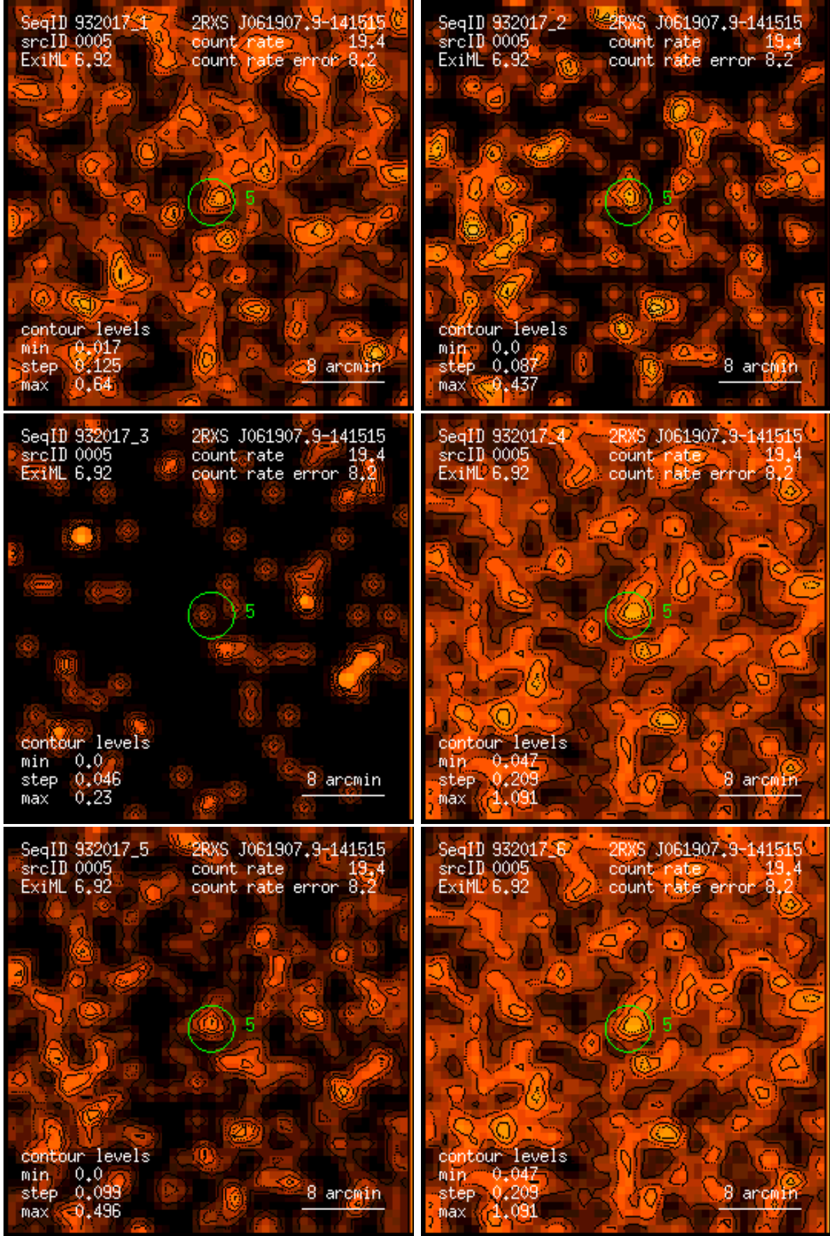
Figure 5: RASS 932017: detection 0005: band rate images, Gaussian filter: (1) PSPC channels 11 – 41, (2) 52 – 90, (3) 91 – 201, (4) 11 – 235, (5) 52 – 201, (6) 11 – 201. Broad band rates in counts/ks. Band rate contour levels in counts/ks/arcmin 2 .
