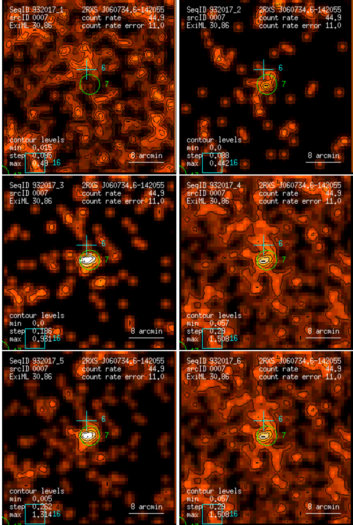
Figure 7: RASS 932017: detection 0007: band rate images, Gaussian filter: (1) PSPC channels 11 – 41, (2) 52 – 90, (3) 91 – 201, (4) 11 – 235, (5) 52 – 201, (6) 11 – 201. Broad band rates in counts/ks. Band rate contour levels in counts/ks/arcmin 2 .
