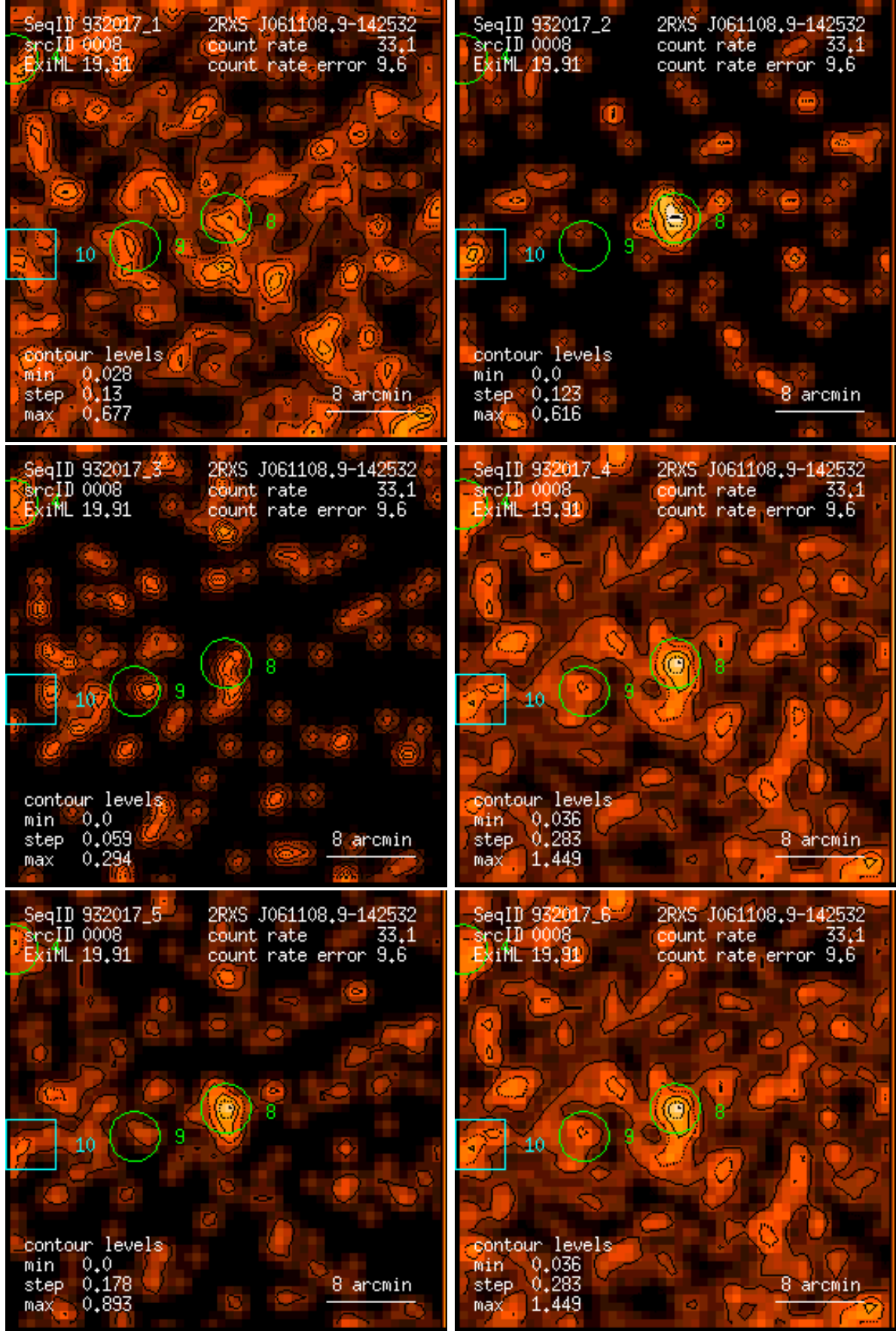
Figure 8: RASS 932017: detection 0008: band rate images, Gaussian filter: (1) PSPC channels 11 – 41, (2) 52 – 90, (3) 91 – 201, (4) 11 – 235, (5) 52 – 201, (6) 11 – 201. Broad band rates in counts/ks. Band rate contour levels in counts/ks/arcmin 2 .
