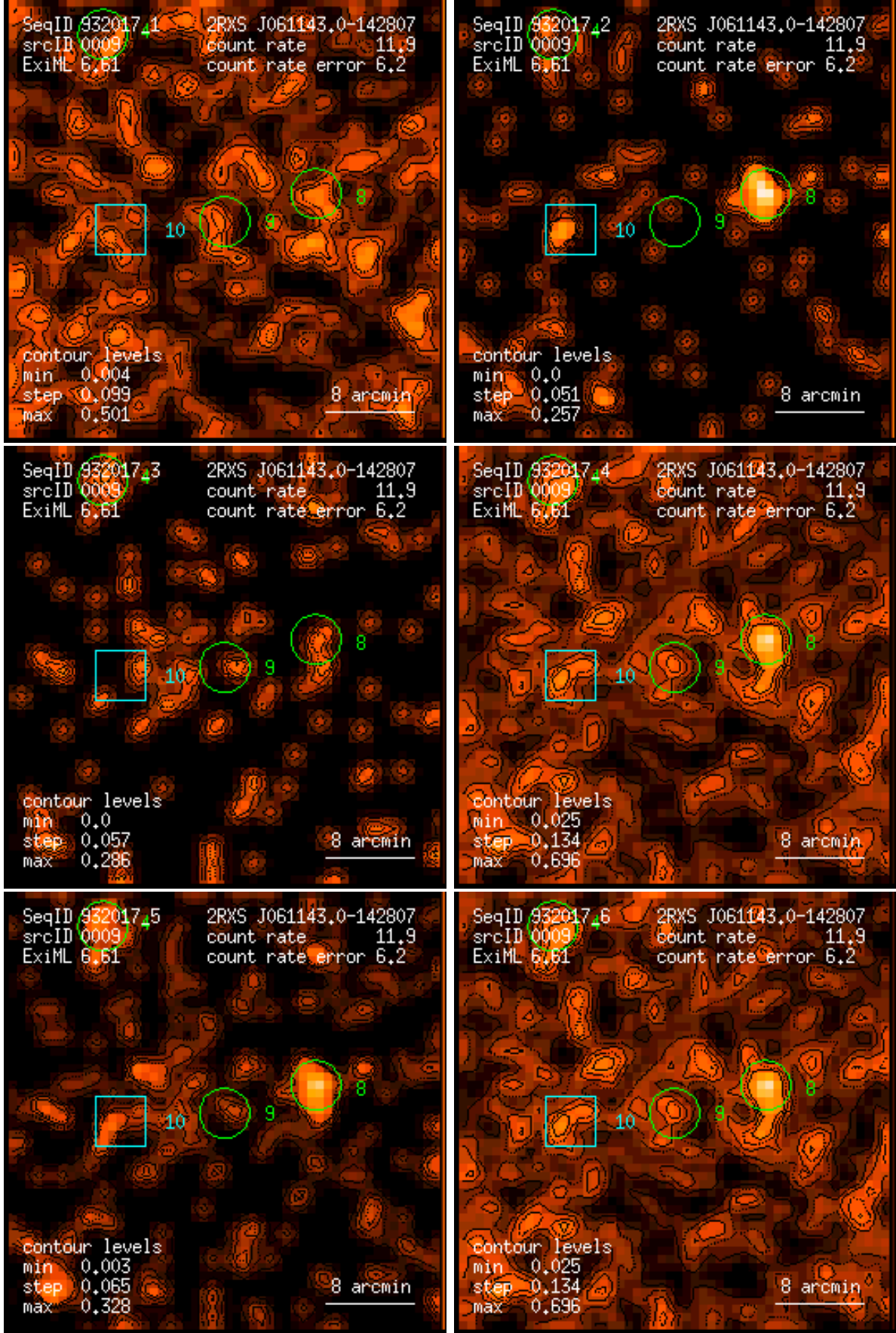
Figure 9: RASS 932017: detection 0009: band rate images, Gaussian filter: (1) PSPC channels 11 – 41, (2) 52 – 90, (3) 91 – 201, (4) 11 – 235, (5) 52 – 201, (6) 11 – 201. Broad band rates in counts/ks. Band rate contour levels in counts/ks/arcmin 2 .
