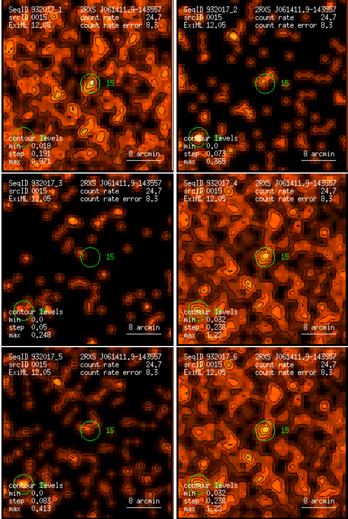
Figure 15: RASS 932017: detection 0015: band rate images, Gaussian filter: (1) PSPC channels 11 – 41, (2) 52 – 90, (3) 91 – 201, (4) 11 – 235, (5) 52 – 201, (6) 11 – 201. Broad band rates in counts/ks. Band rate contour levels in counts/ks/arcmin 2 .
