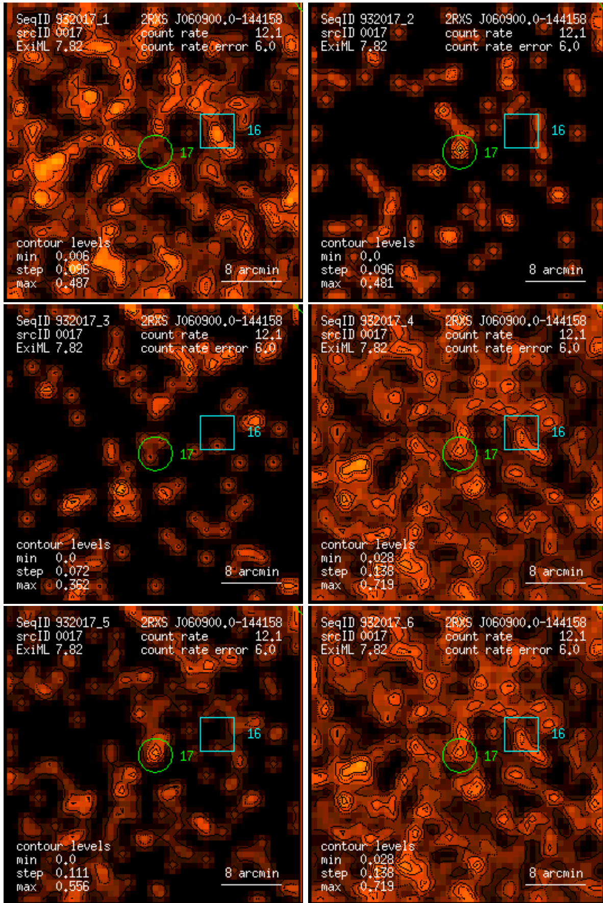
Figure 17: RASS 932017: detection 0017: band rate images, Gaussian filter: (1) PSPC channels 11 – 41, (2) 52 – 90, (3) 91 – 201, (4) 11 – 235, (5) 52 – 201, (6) 11 – 201. Broad band rates in counts/ks. Band rate contour levels in counts/ks/arcmin 2 .
