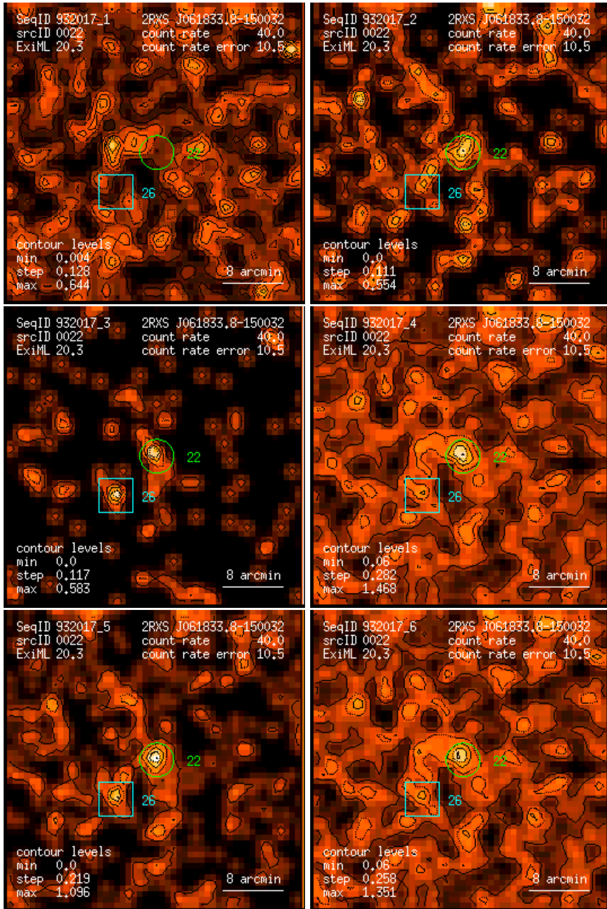
Figure 22: RASS 932017: detection 0022: band rate images, Gaussian filter: (1) PSPC channels 11 – 41, (2) 52 – 90, (3) 91 – 201, (4) 11 – 235, (5) 52 – 201, (6) 11 – 201. Broad band rates in counts/ks. Band rate contour levels in counts/ks/arcmin 2 .
