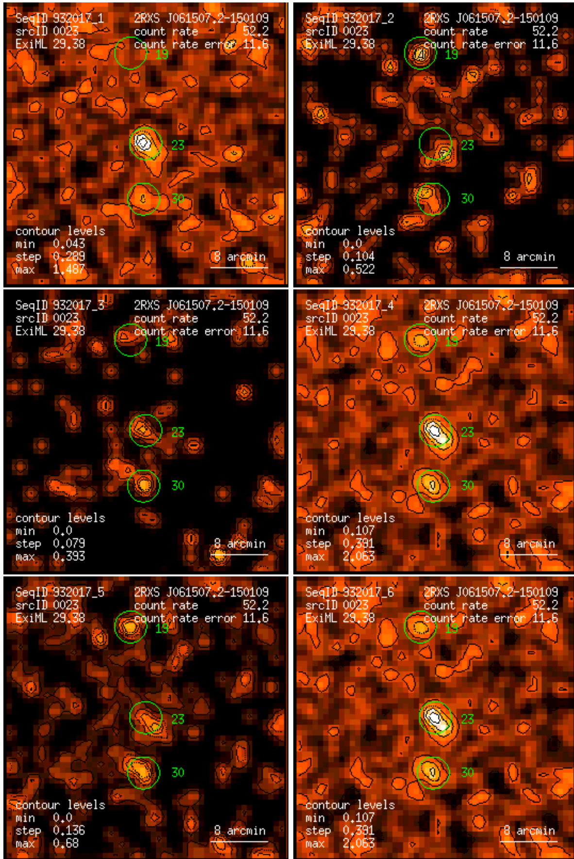
Figure 23: RASS 932017: detection 0023: band rate images, Gaussian filter: (1) PSPC channels 11 – 41, (2) 52 – 90, (3) 91 – 201, (4) 11 – 235, (5) 52 – 201, (6) 11 – 201. Broad band rates in counts/ks. Band rate contour levels in counts/ks/arcmin 2 .
