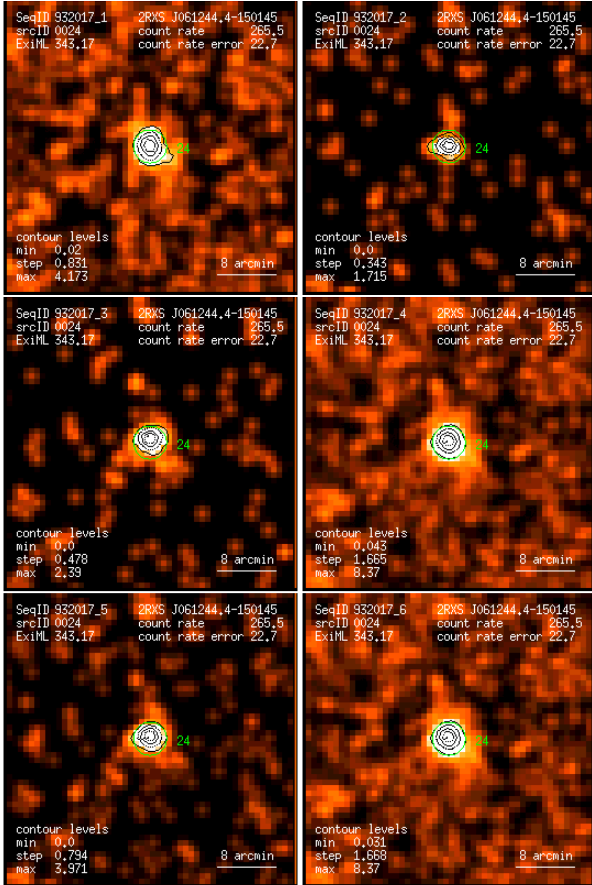
Figure 24: RASS 932017: detection 0024: band rate images, Gaussian filter: (1) PSPC channels 11 – 41, (2) 52 – 90, (3) 91 – 201, (4) 11 – 235, (5) 52 – 201, (6) 11 – 201. Broad band rates in counts/ks. Band rate contour levels in counts/ks/arcmin 2 .
