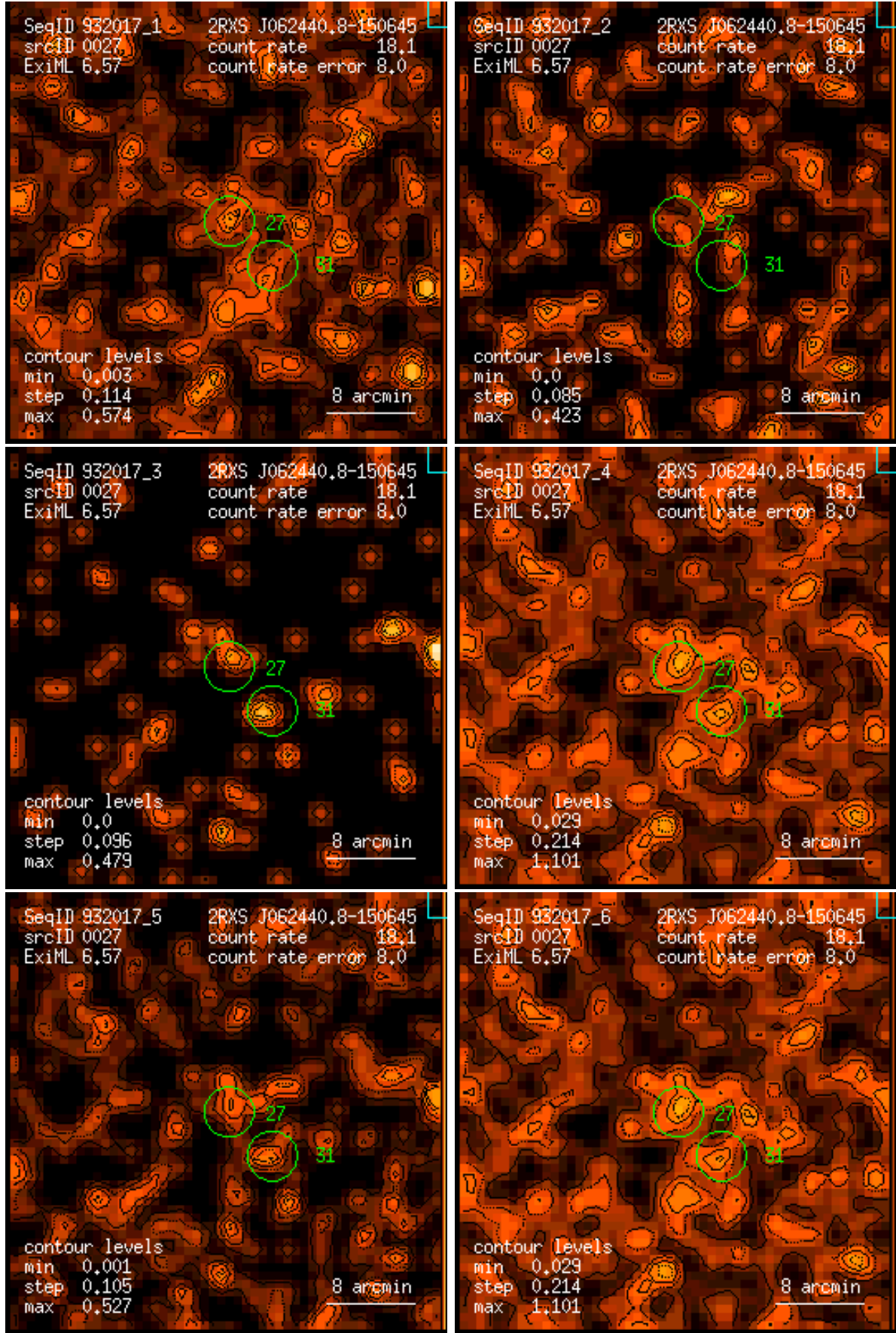
Figure 27: RASS 932017: detection 0027: band rate images, Gaussian filter: (1) PSPC channels 11 – 41, (2) 52 – 90, (3) 91 – 201, (4) 11 – 235, (5) 52 – 201, (6) 11 – 201. Broad band rates in counts/ks. Band rate contour levels in counts/ks/arcmin 2 .
